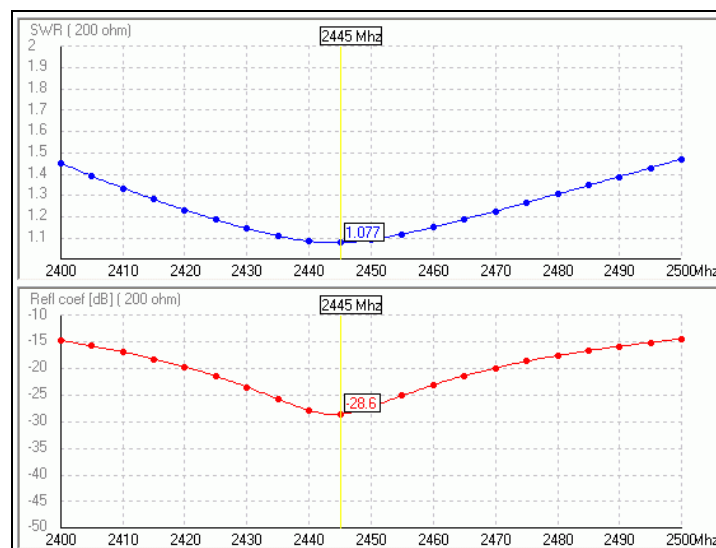
Input matching of Amos antenna
