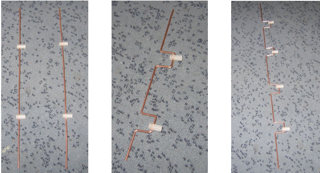
Building of radiating elements of Amos antenna
