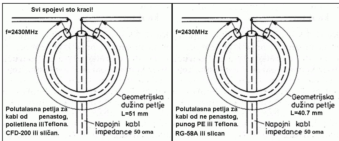
Half wave balun physical lenght depending on coaxial calbe type and its connection
