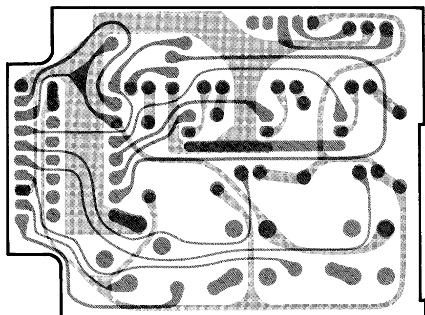
Obverse View of Solder Side
