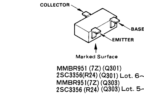
Obverse View of Solder Side
