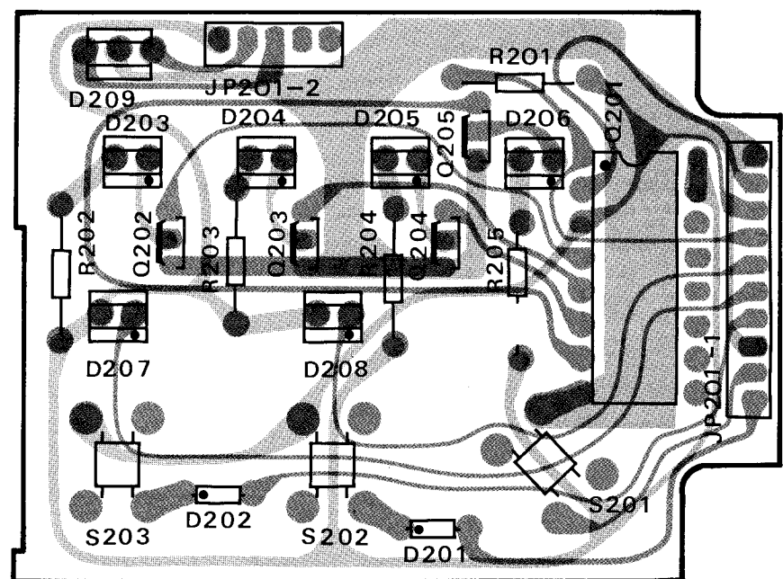
Obverse View of Component Side
