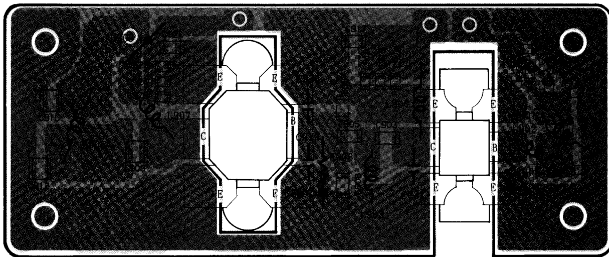
Obverse View of "Mixed Component" Side
