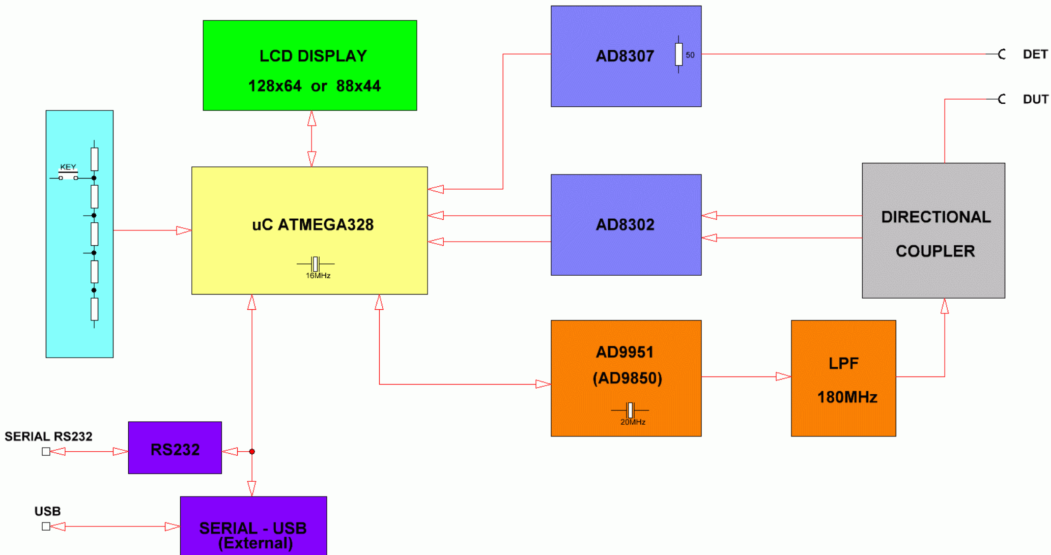
VNA IZ1PMX - BLOCK DIAGRAM
