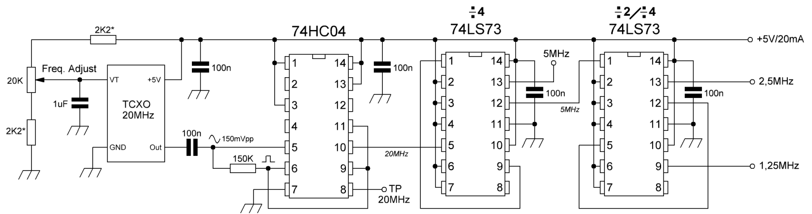
Time Base Oscillator 20/5/2,5/1,25 MHz
