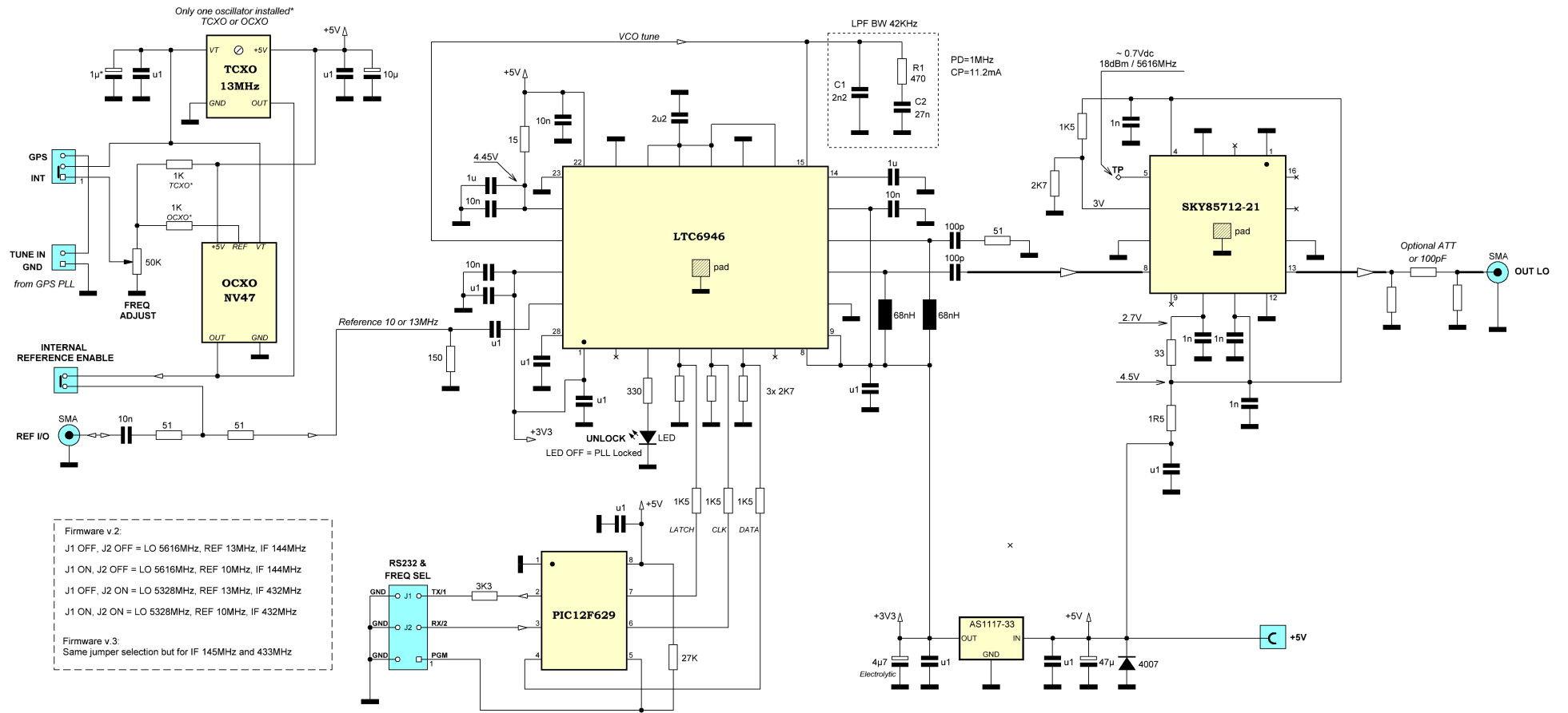
PLL OSCILLATOR FOR 5,76GHz TRANSVERTER YO4HFU rev.4.1
