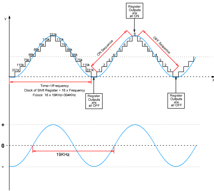
Pilot Tone synthesized by 8 bit Shift Register
