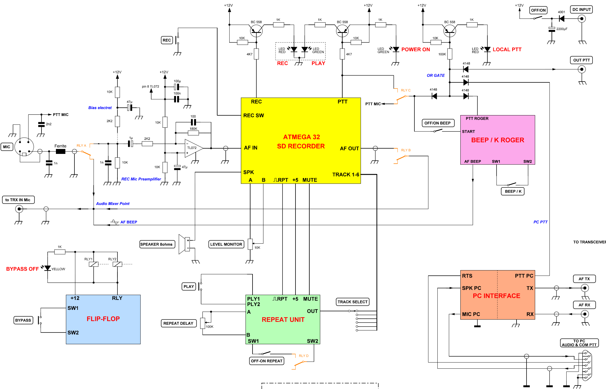
DIGITAL AUDIO RECORDER BLOCK DIAGRAM YO4HFU @ 2011
