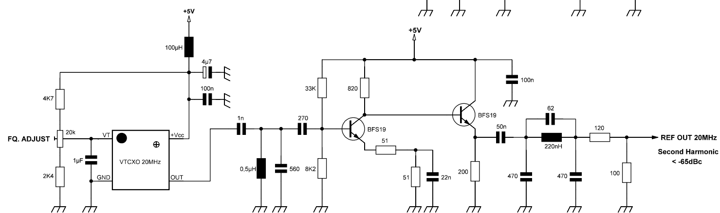
1GHz Fractional-N PLL SA7025 Pastorcici Robert - 2013 YO4HFU
