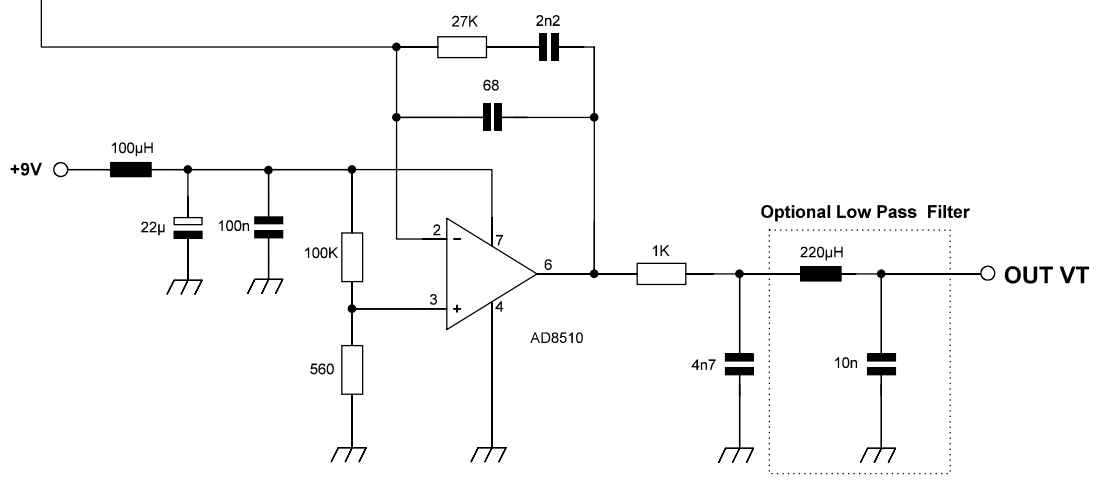
PLL UHF LMX2324 Pastorcici Robert 02.2013
