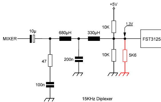
15KHz Diplexer
