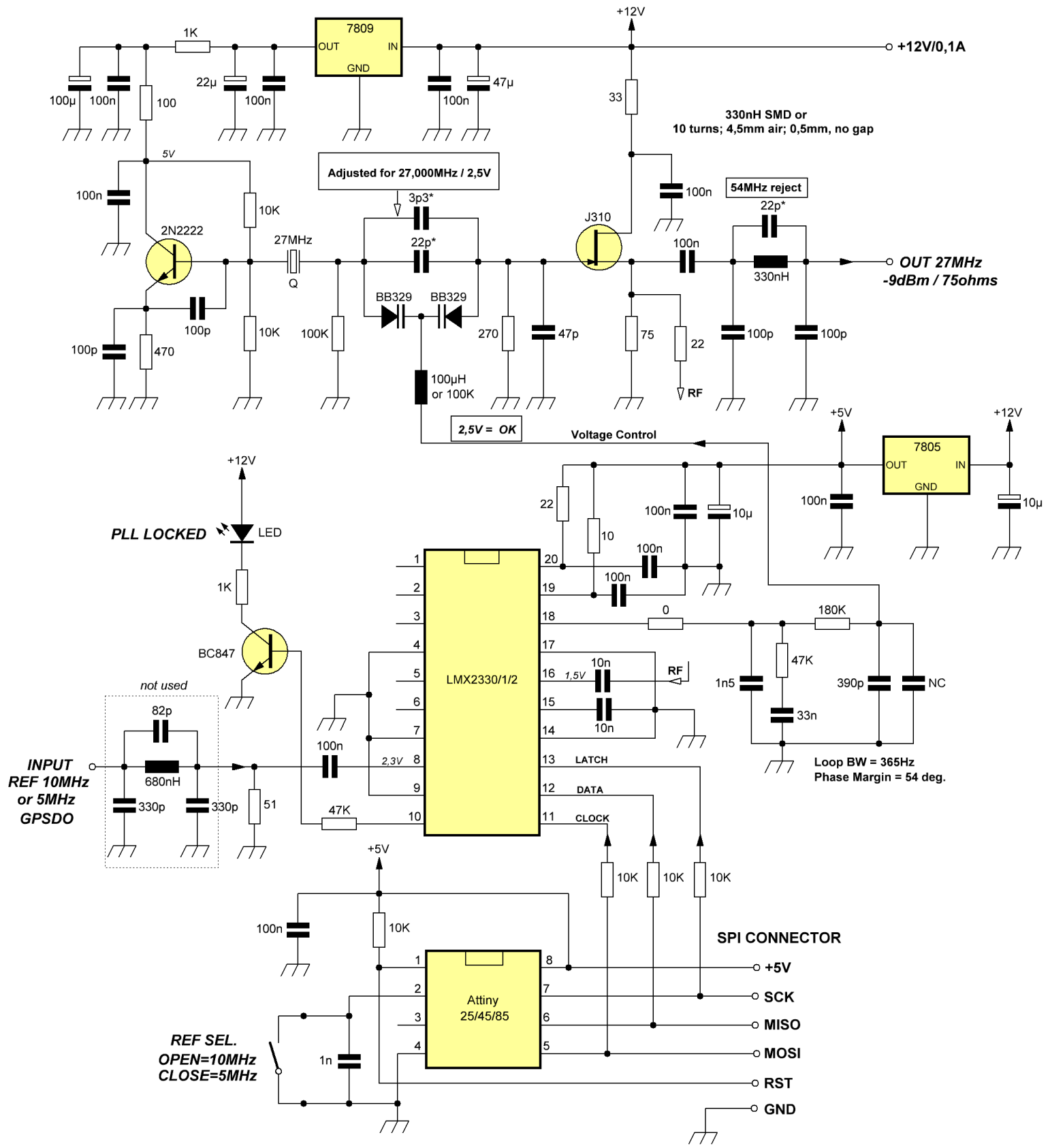
PLL 27MHz for LNB Reference rev 1.2 / 26.01.2017 YO4HFU
