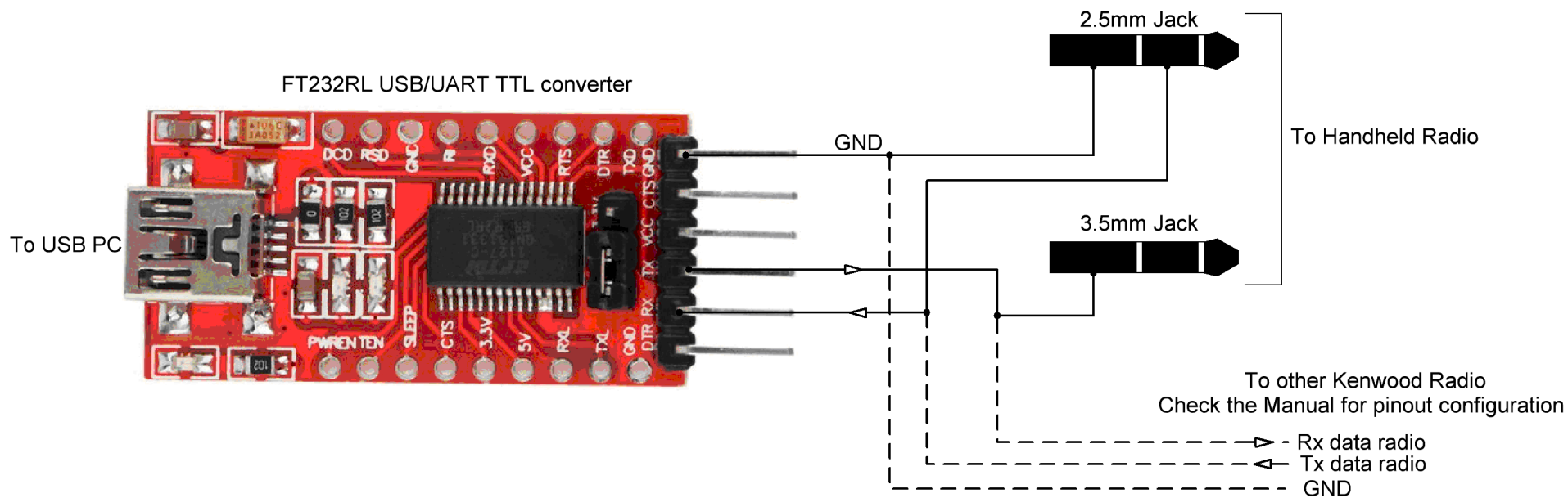
Universal USB programming cable for Kenwood Radio yo4hfu - 2018
