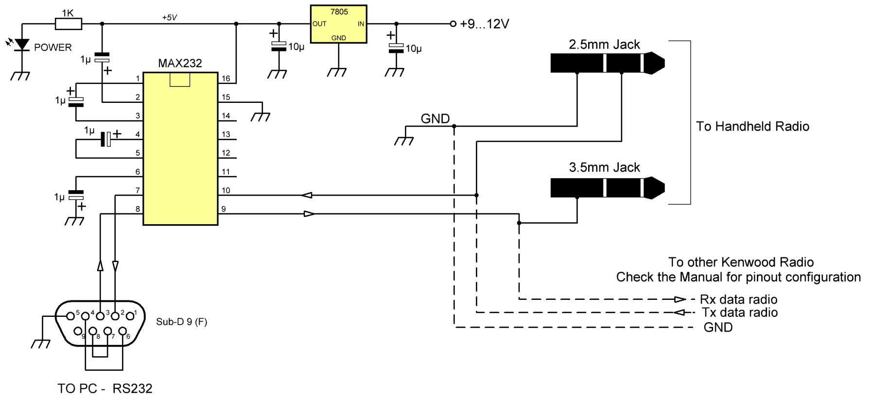
Universal RS232 programming cable for Kenwood Radio yo4hfu - 2018
