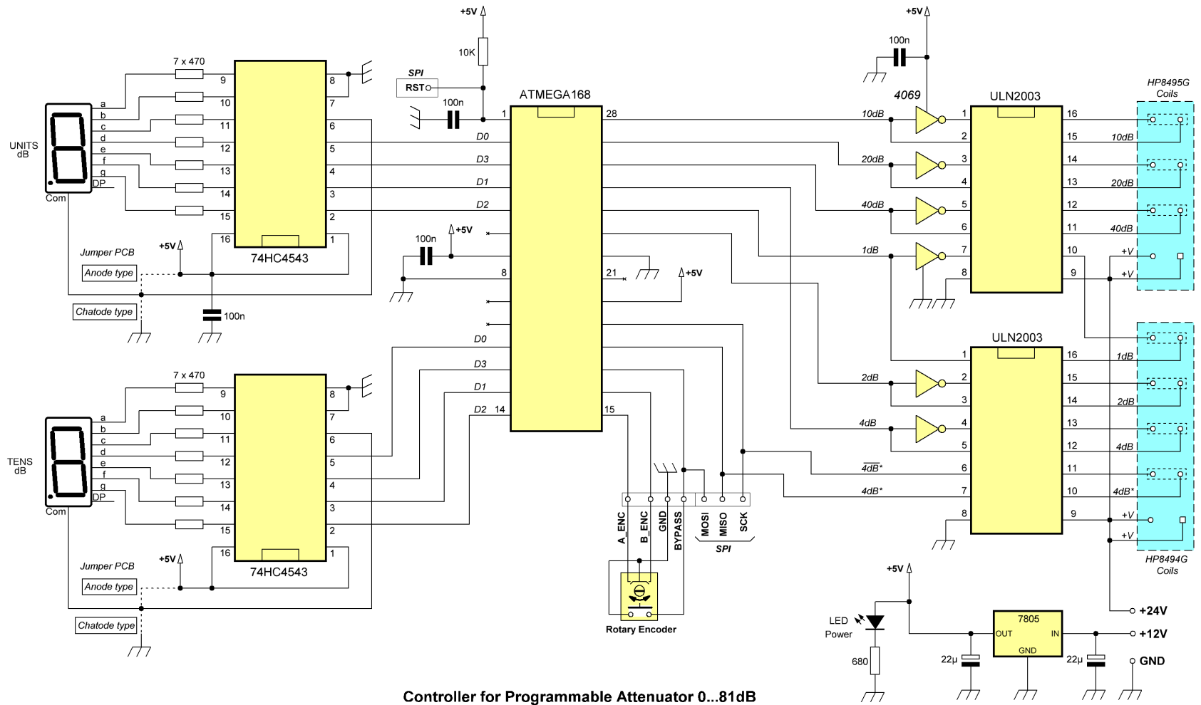
Controller for Programmable Attenuator 0...81dB
