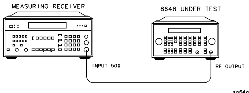
Figure 8-3. FM Accuracy Equipment Setup for Option 1E2
