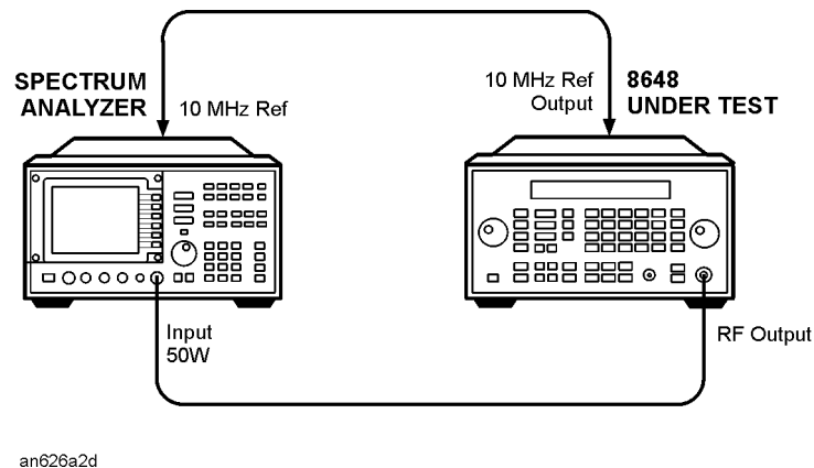
Figure 8-13. Harmonics Equipment Setup
