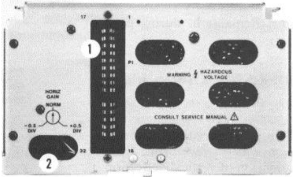
Figure 3-2. Rear Panel Controls and Connectors (1 of 2)
