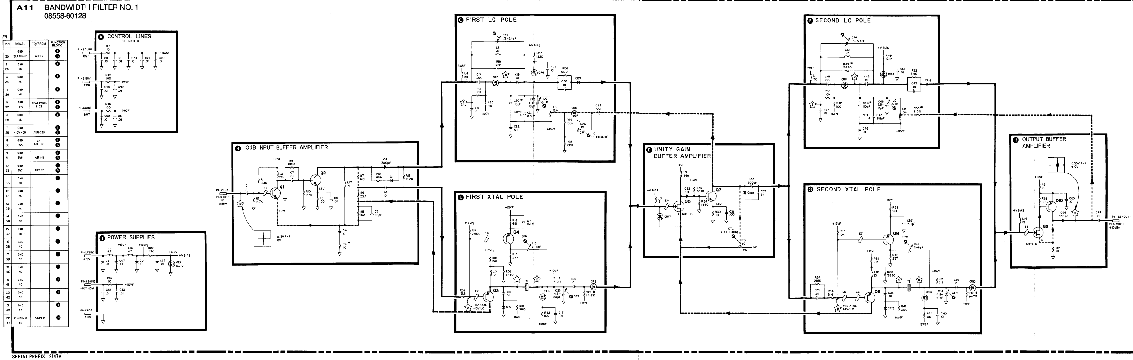
Figure 8-30. A11 Bandwidth Filter No. 1, Schematic
