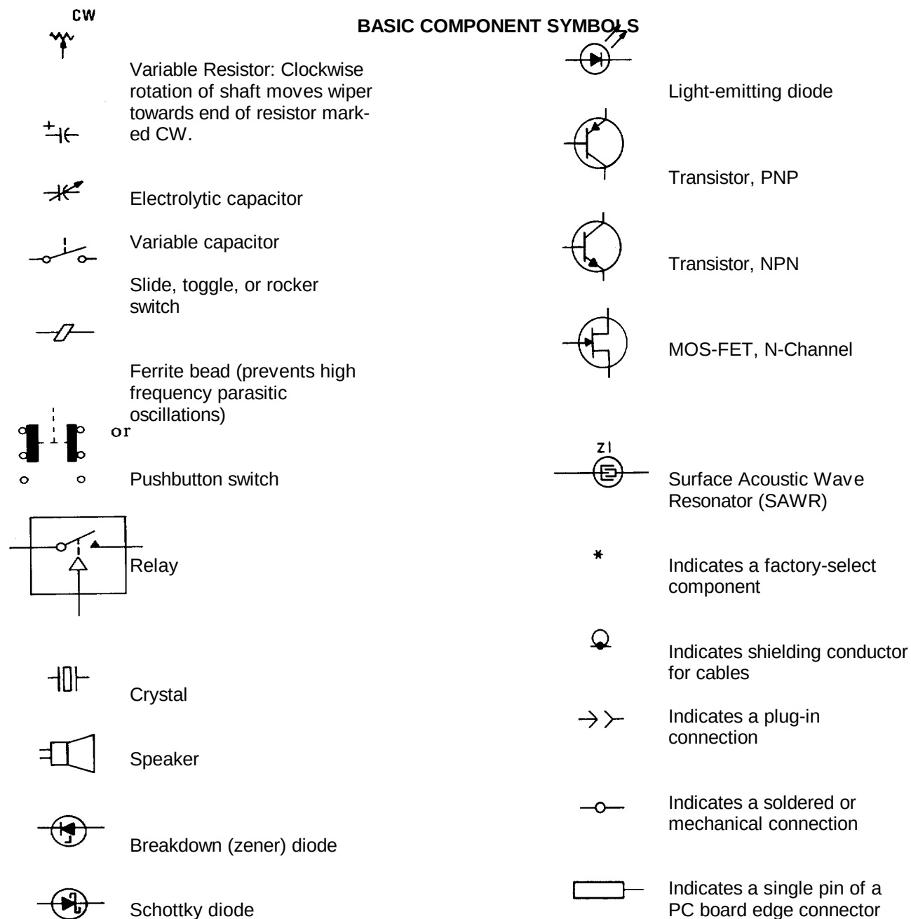
Figure 8-1. Symbols Used in Schematics and Block Diagrams (1 of 4)
