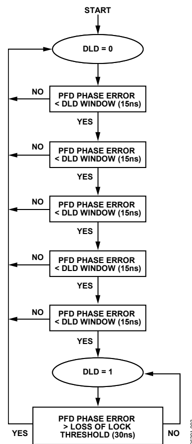
Figure 2. State Diagram for Digital Lock Detect (Lock Detect Precision (LDP) is 5 in This Case)
