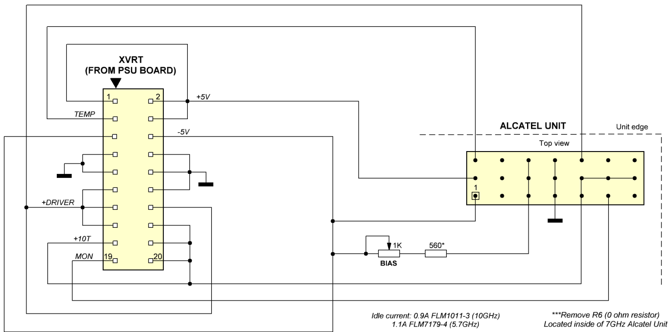
ALCATTEL XVRT 21 PIN ADAPTER TO PSU BOARD Vers. 1.0 YO4HFU - 2021
