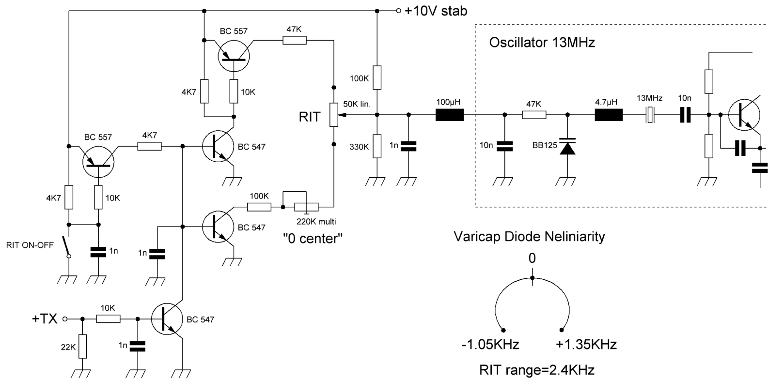
RIT CONTROL FOR VFO-PLL YO4HFU - 2006
