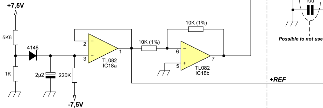
Diode Clipper for 38KHz DSB Temperature Compensated Voltage Reference
