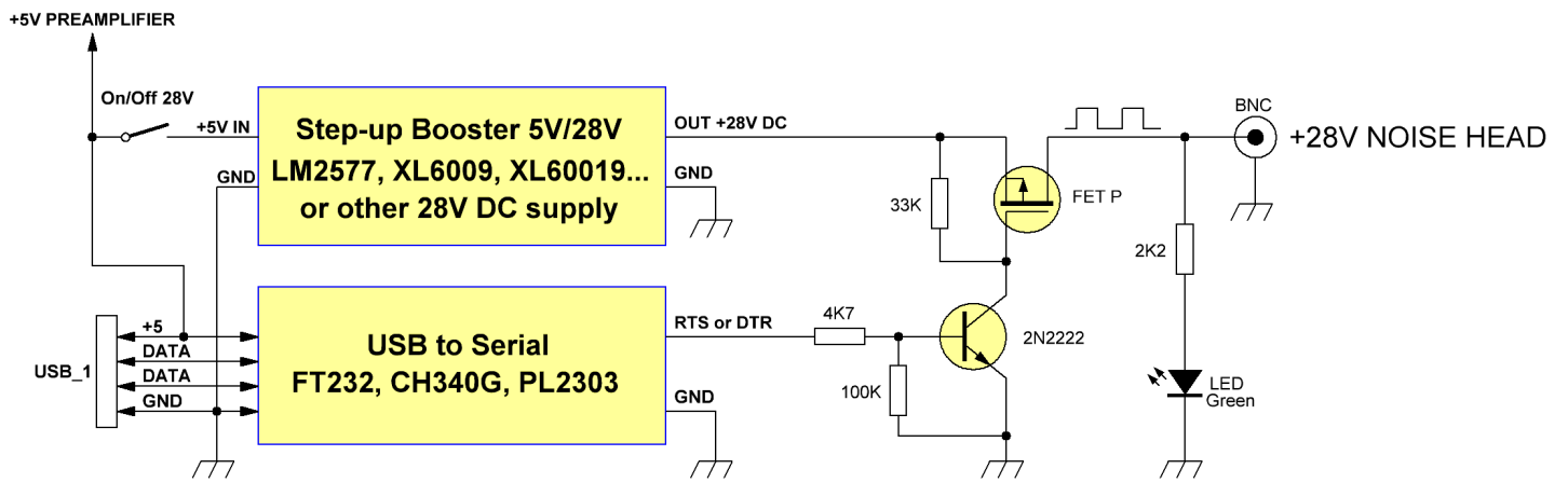
CANFI 28V Switch - YO4HFU
