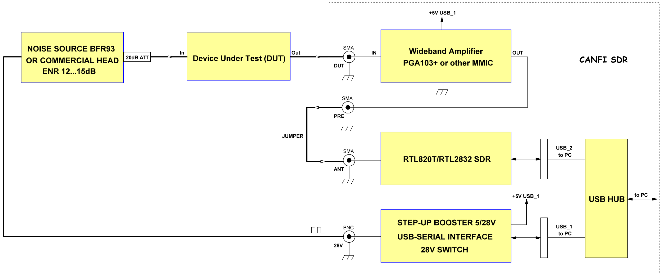
CANFI SDR BLOCK DIAGRAM - YO4HFU
