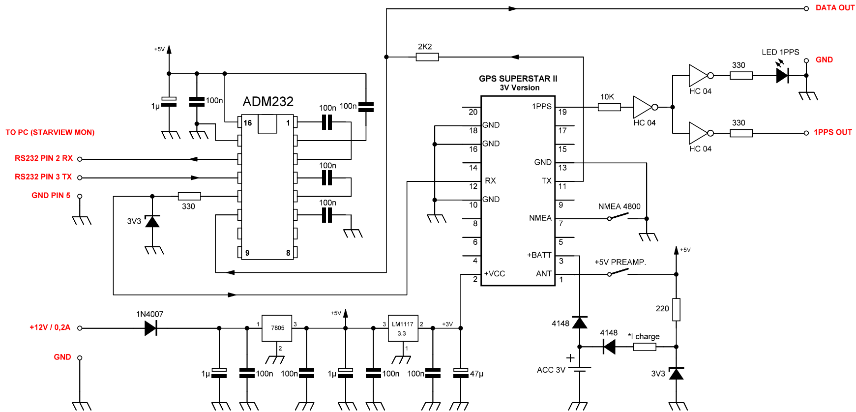
GPS SUPERSTAR II ARDUINO ROTATOR YO4HFU 2014
