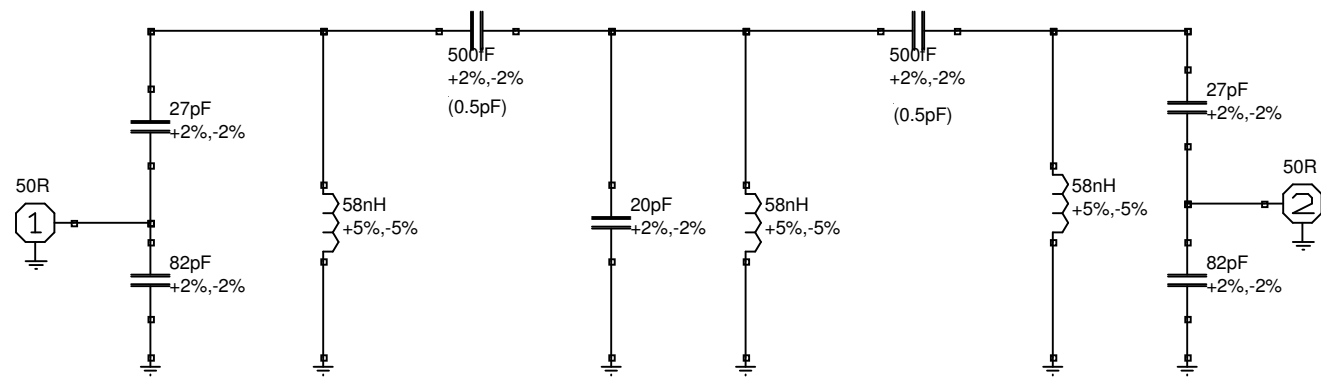
BAND PASS FILTER 144MHZ
