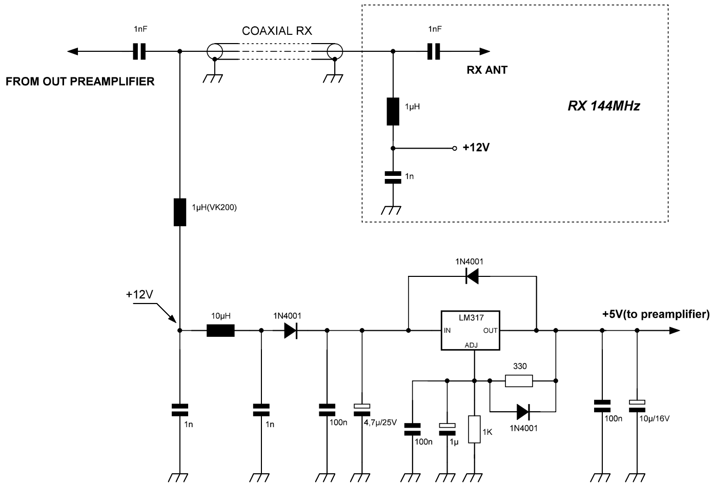
LOW NOISE POWER SUPPLY FOR ATF54143 YO4HFU
