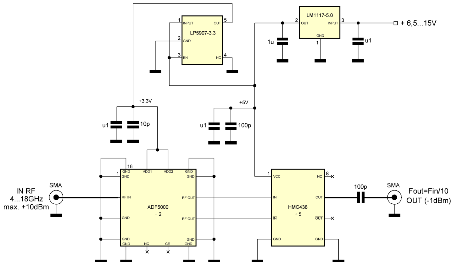
ADF5000 microwave prescaler by 10 YO4HFU
