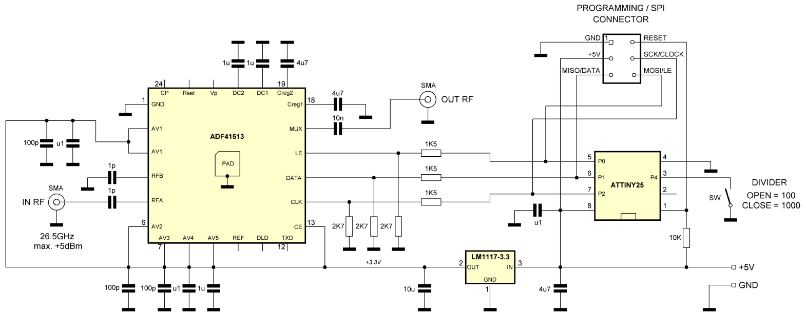
ADF41513 PRESCALER YO4HFU
