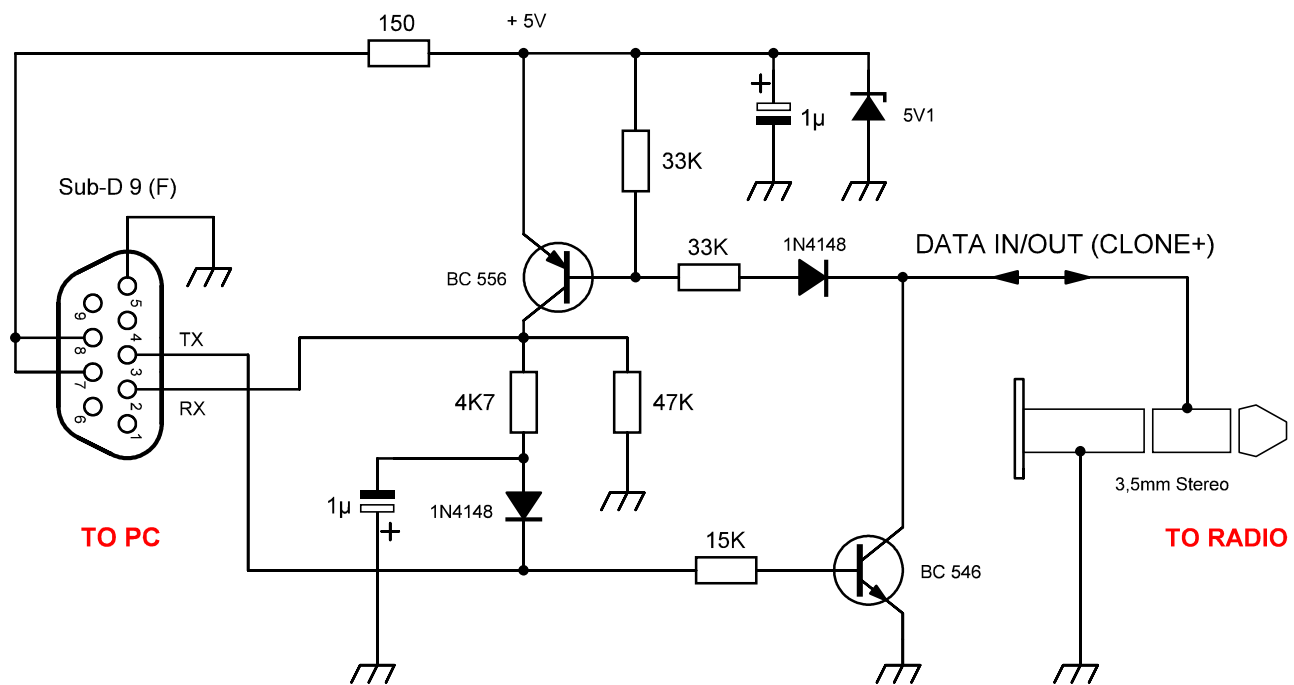
ICOM PROGRAMMING INTERFACE - OPC478 YO4HFU @ 2012
