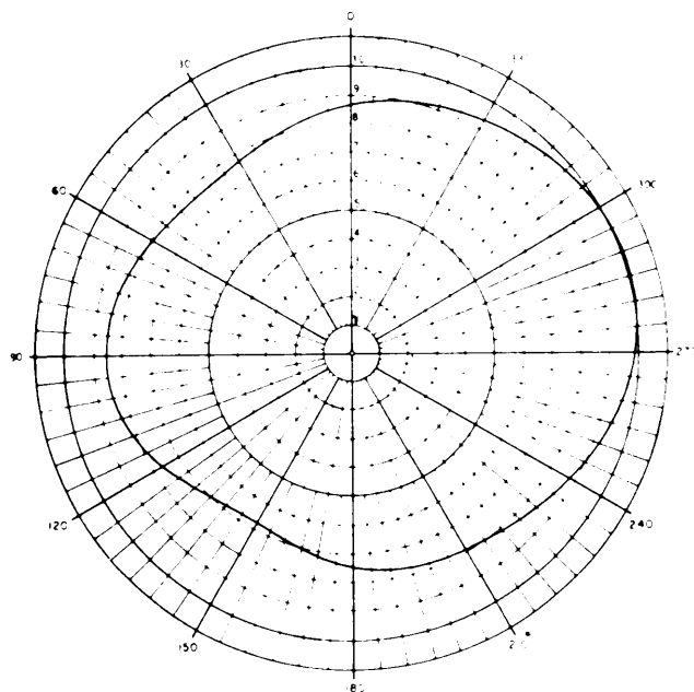
Figure 3-18. 15. 5-MHz Azimuth Plane Pattern, Average Ground.
