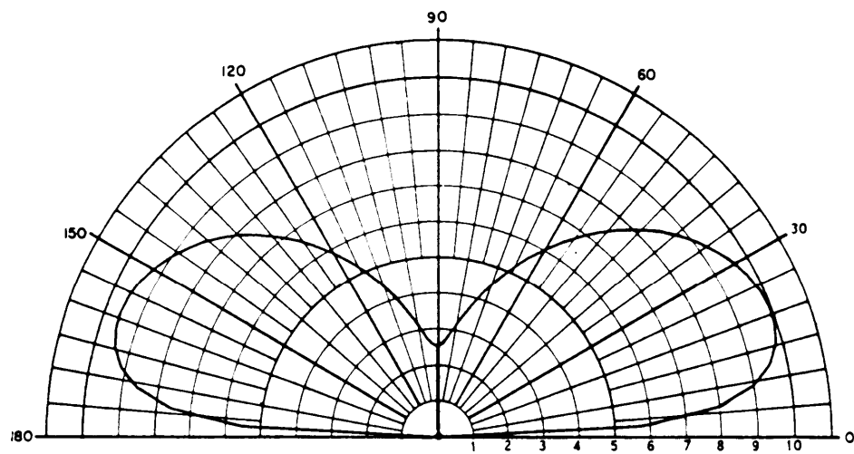
Figure 3-13. 2.5-MHz Elevation Plane Pattern, Average Ground.
