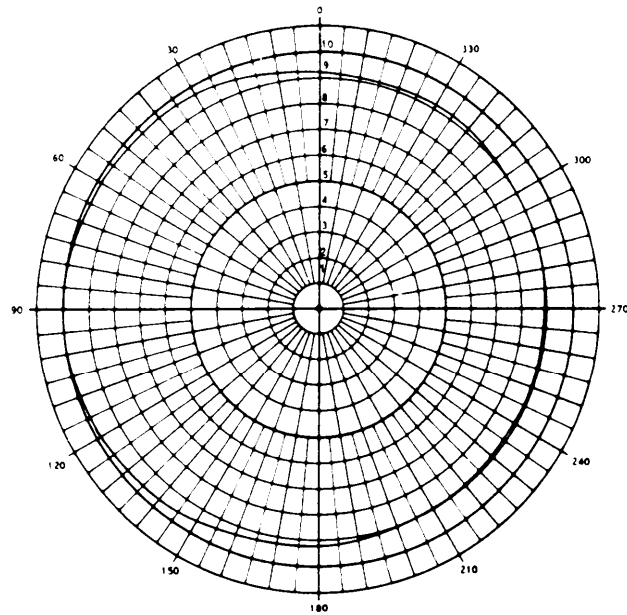
Figure 3-12. 2.5-MHz Azimuth Plane Pattern, Average Ground.
