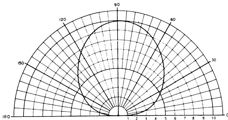
Figure 3-19. 15.5-MHz Elevation Plane Pattern, Average Ground.
