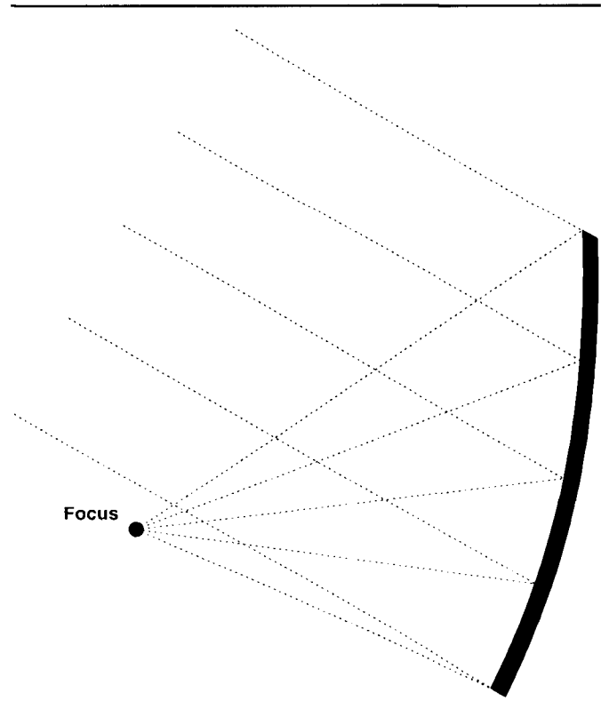
Fig 2—An offset-fed parabolic dish antenna aimed at a satellite.
