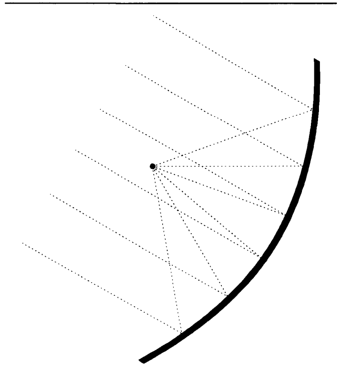
Fig 1—A parabolic dish antenna aimed at a satellite.
