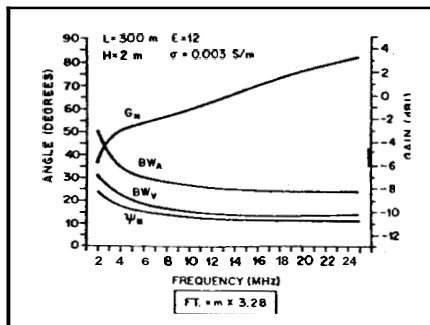
Fig. 7 — Design Parameters for average dry soil: H = 6.5 ft; L = 984 ft.
