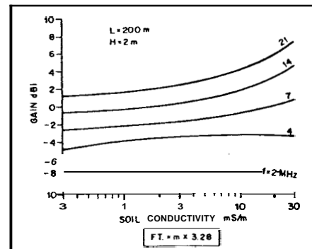
Fig. 10 — Gain of a Beverage antenna element as a function of frequency and conductivity ( L = 656 ft; H = 6.5 ft).
