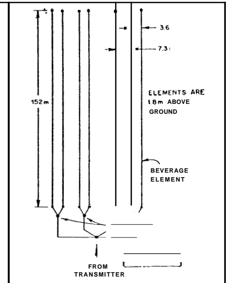
Fig. 11 — Plane view of an experimental Beverage array. See text for details.
