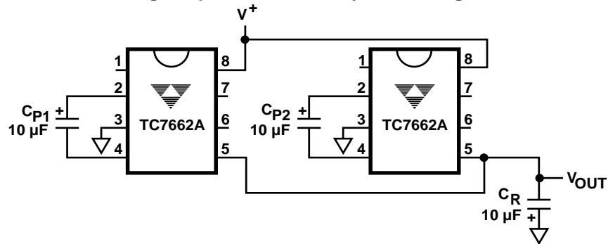
Positive Voltage Multiplier
