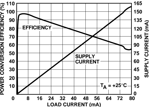
Power Conversion Efficiency vs I_{LOAD}
