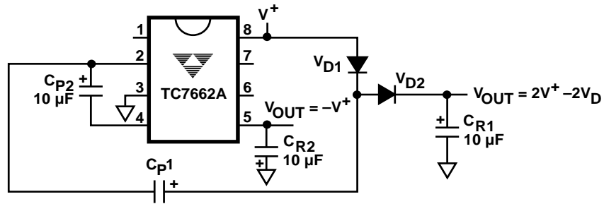
Combined Negative Converter and Positive Multiplier
