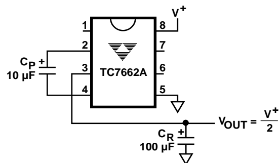
Split V^+ In Half
