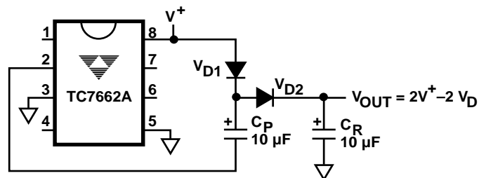
Positive Voltage Multiplier
