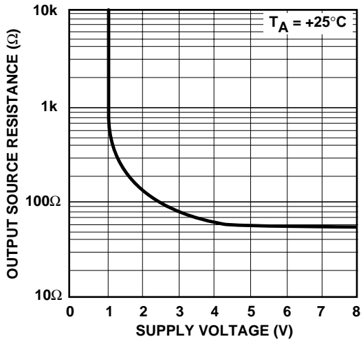
Output Source Resistance vs. Supply Voltage
