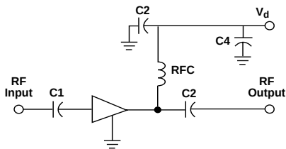
Figure 15. Schematic Diagram.
