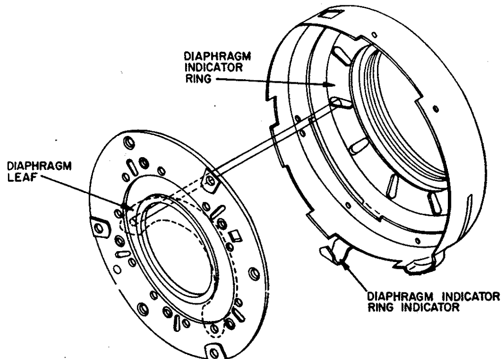
Figure 6. DIAPHRAGM OPERATION
