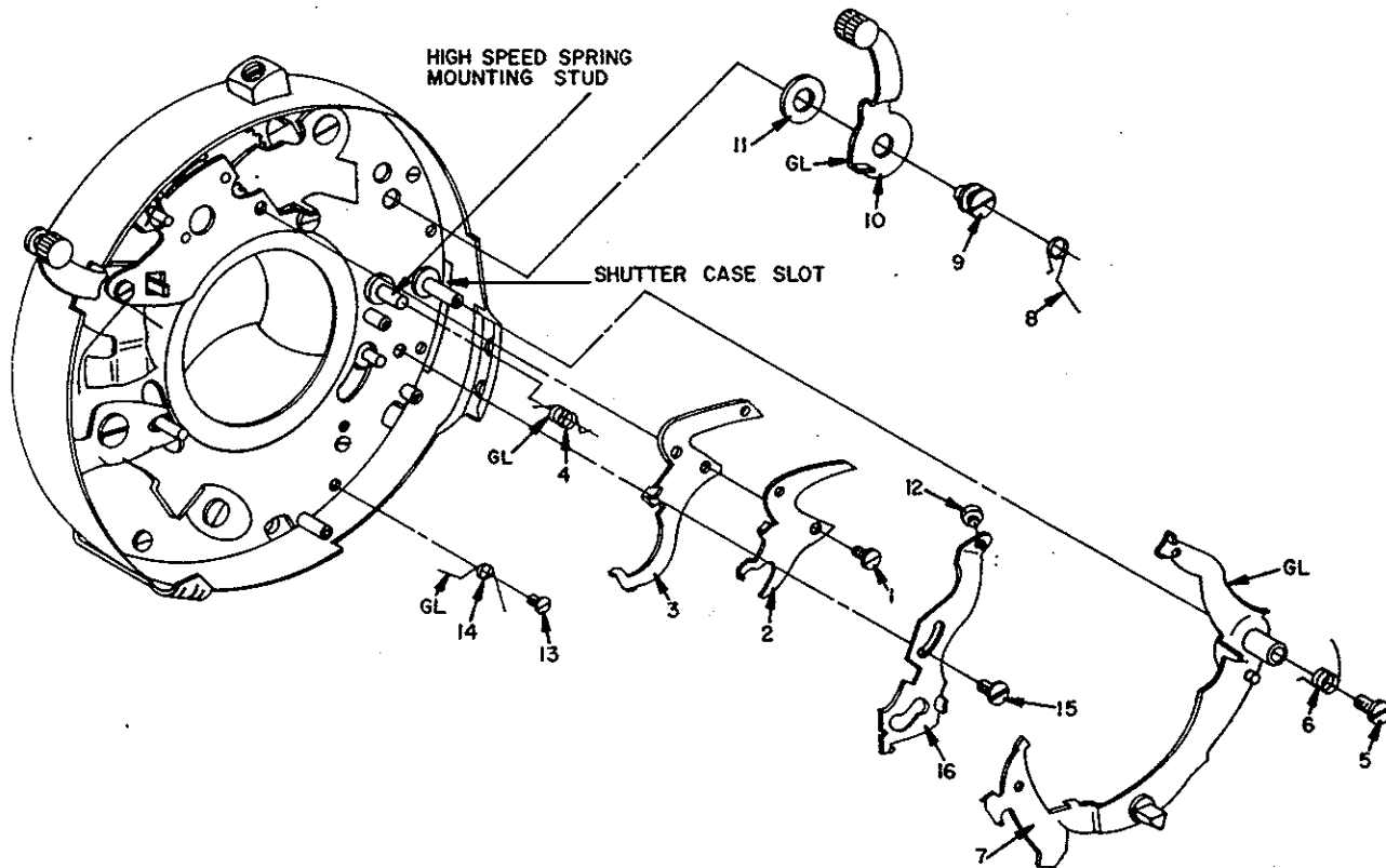
Figure 11. NO. 1 SHUTTER, DISASSEMBLY - STAGE 4
