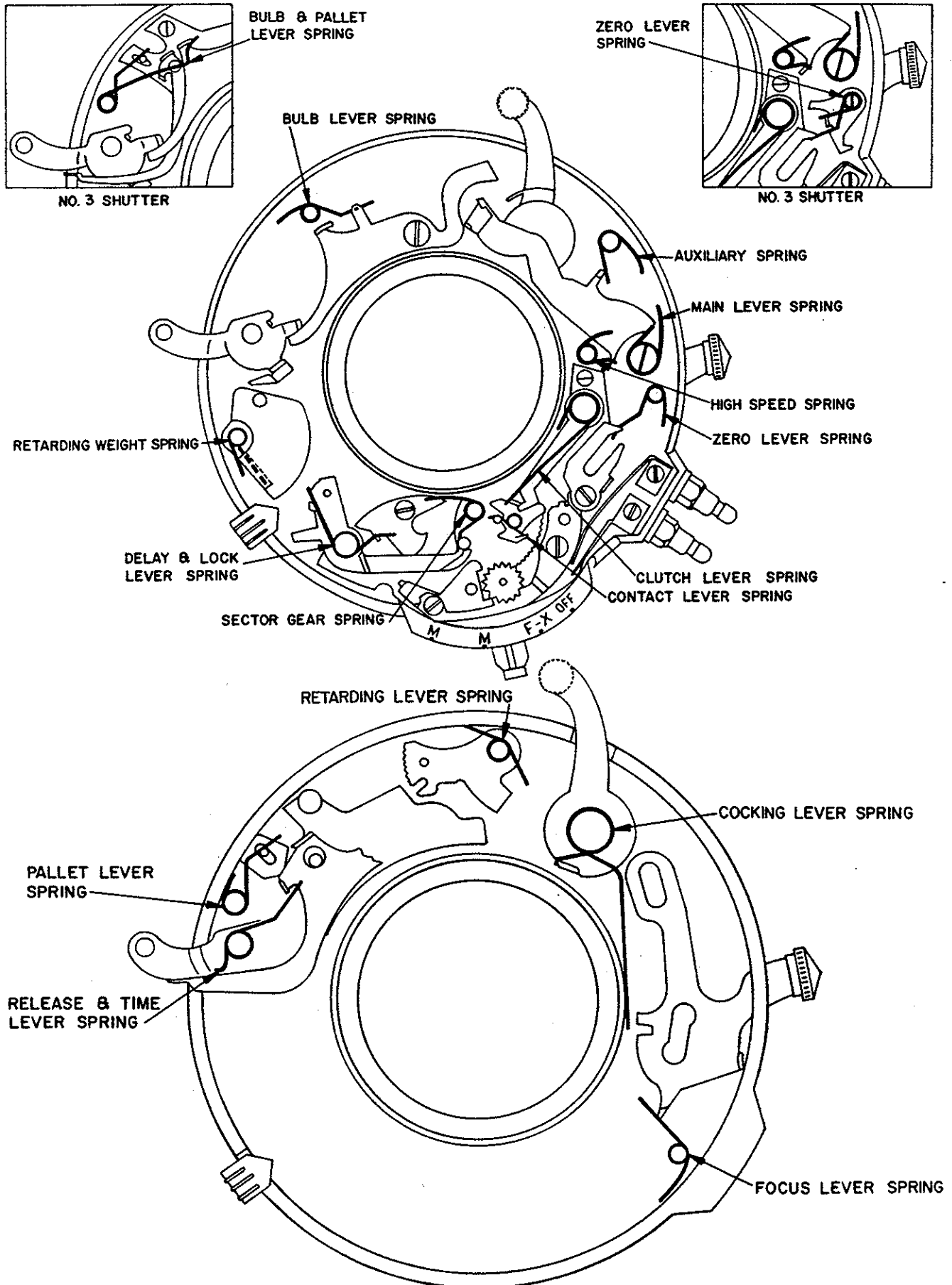
Figure 21. NO. 2 AND 3 SHUTTER, SPRING POSITIONS
