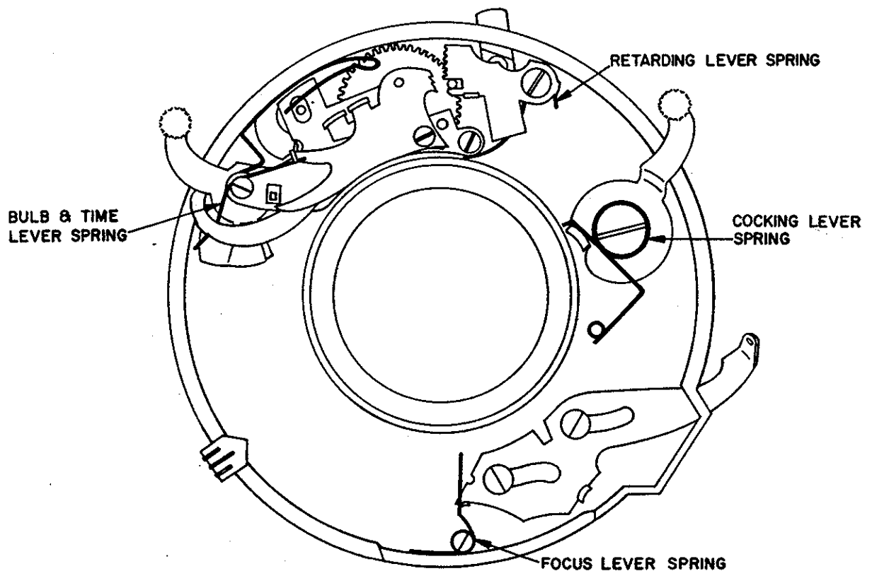
Figure 20. NO. 1 SHUTTER, SPRING POSITIONS
