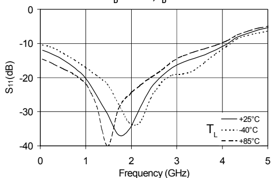
|S_{11}| vs. Frequency V_D = 4.9 V, I_D = 80 mA
