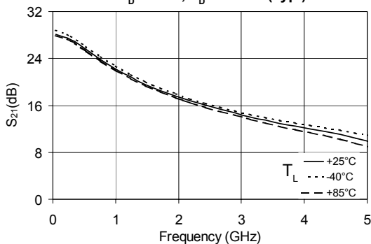
|S_{21}| vs. Frequency V_D = 4.9 V, I_D = 80 mA (Typ.)
