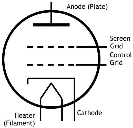
Vacuum Tube
