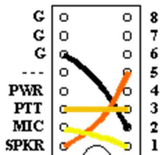
Figure 6. Internal jumper board wiring for the Yaesu FT-8900 rear 6-pin mini-DIN connector cable
