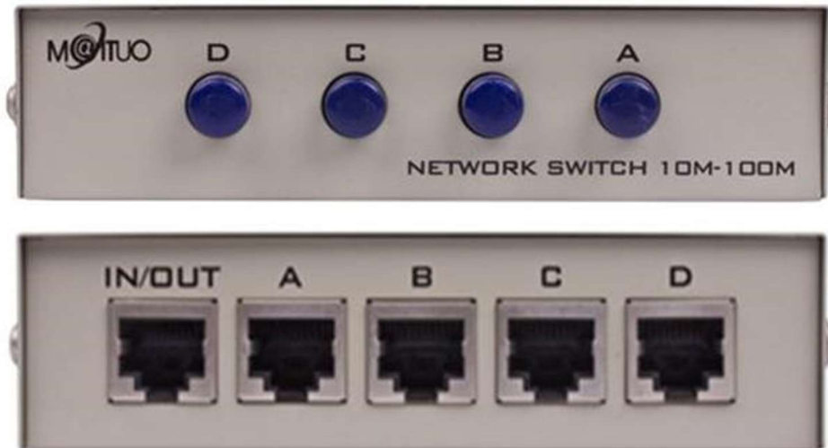
Figure 14. Network data switch for selecting which transceiver connects with Signalink
