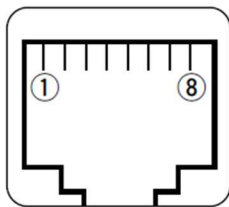
Figure A-1. Front panel view of the RJ-45 microphone jack with pin assignments for accessible signals; note that three of the four signals essential for the SignalLink unit (PTT, GND and MIC) are available via this connector. [The fourth essential signal, SPKR, is available from a 3.5mm speaker jack at the rear of the radio.]
