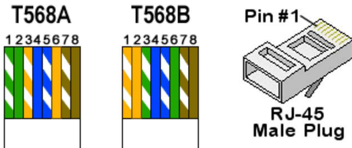
Figure 3. Two most common wire color codes and pin-numbering convention for the RJ-45 connector
