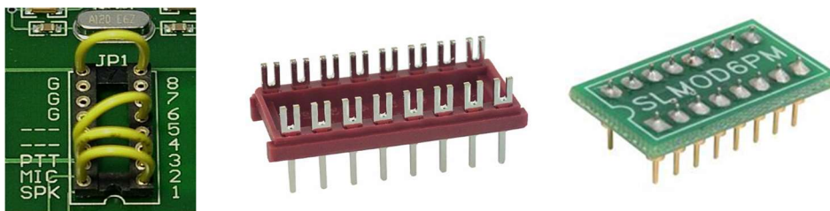
Figure 4. Internal jumper board options for Signalink USB; rightmost photo is a sample of a prewired PCB that can be ordered for a specific transceiver (along with a compatible cable) and is the recommended option
