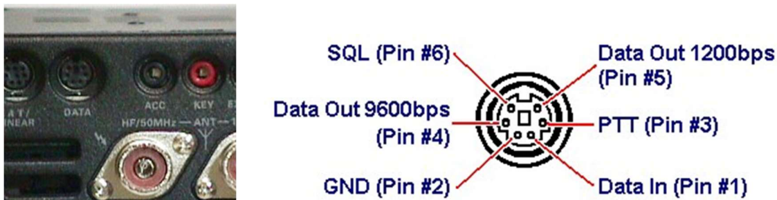
Figure 13. FT-897 6-pin mini-DIN data connector and pin assignments (Pins 1, 2, 3 and 5 are of interest.)
