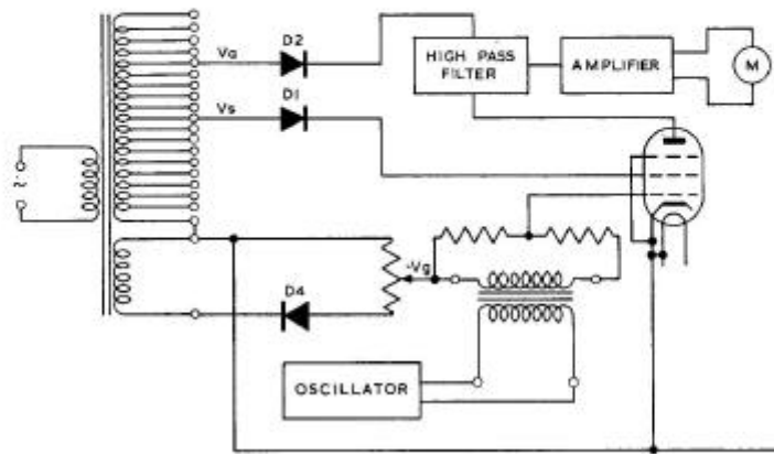
FIGURE 1 Basic Circuit for Mutual Conductance measurement
