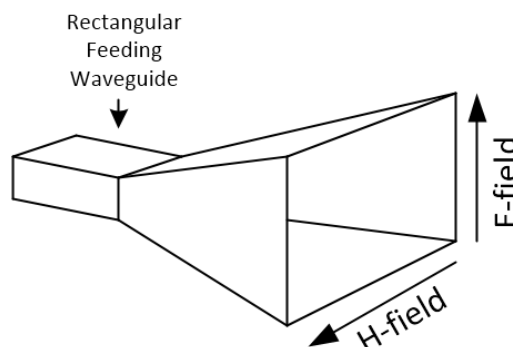
Pyramidal Horn Antenna E-field and H-field directions
