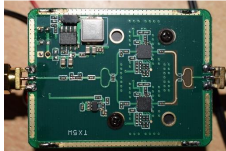
5.8GHz 2W Power Amplifier made with two SiGe-5004L in parallel
