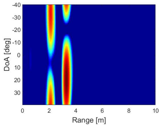
Range-angle representation of two targets placed at 2.1m/-35° respectively at 3.3m/20°
