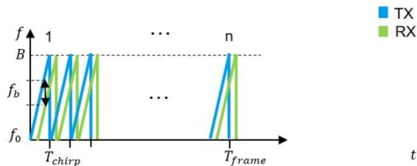
Chirp Sequence using very short sawtooth chirps transmitted in blocks (frames)
