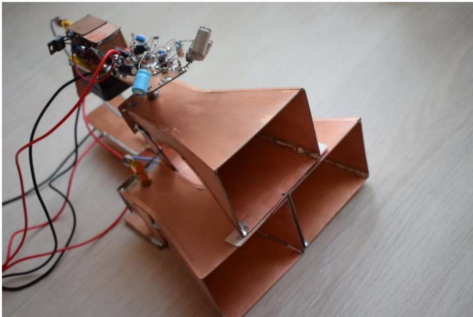
Prototype of the 5.6GHz FMCW Radar using Pyramidal Horn Antennas
