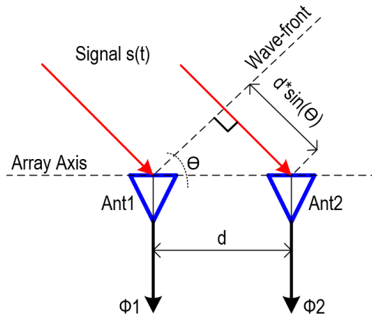
Direction of Arrival using an array with two antenna elements
