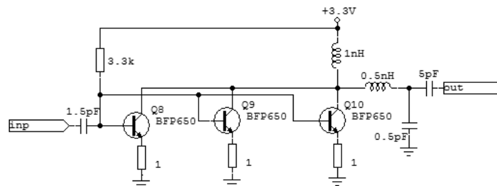
5.6GHz, 0.5W Power Amplifier
