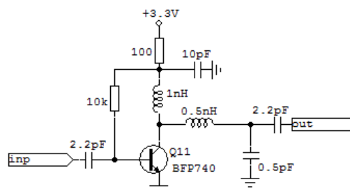
5.6GHz LNA, 16dB Gain and 0.5dB noise figure
