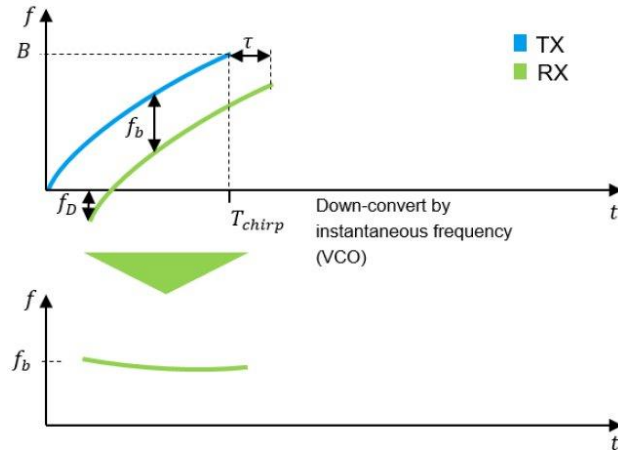
Beat frequency f_b variation due to nonlinear shape of the frequency deviation
