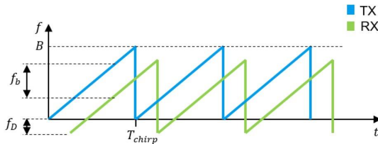
Frequency shift in the echo radar signal due to Doppler effect and range
