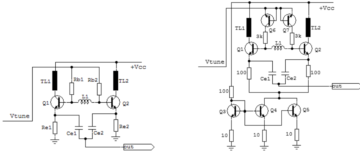
5.6GHz Push-Push VCO – Left: VCO basic circuit – Right: VCO with temperature compensated bias
