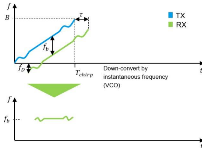
Ripple on TX signal and resulting variation of the beat frequency f_b
