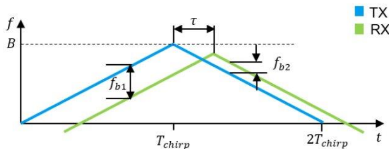
Linear FMCW radar with up-chirp and down-chirp using triangular waveform
