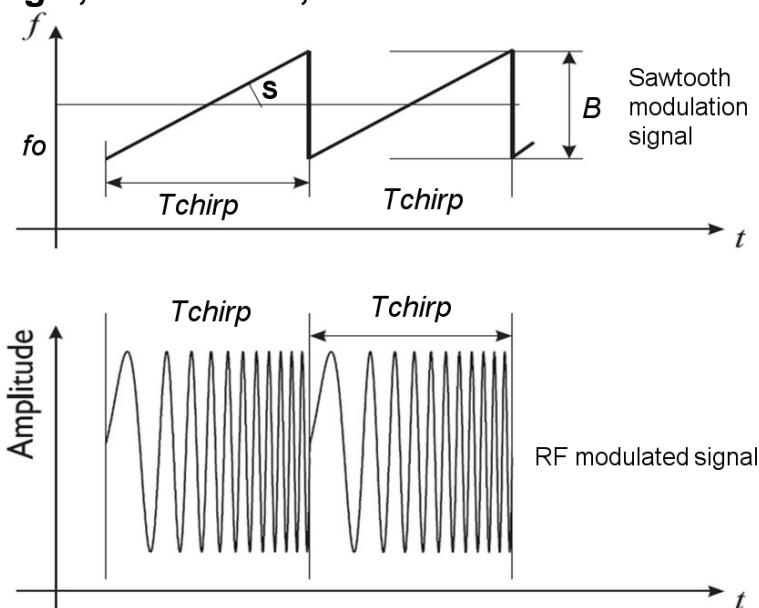
FMCW radar signal using Sawtooth ramp
