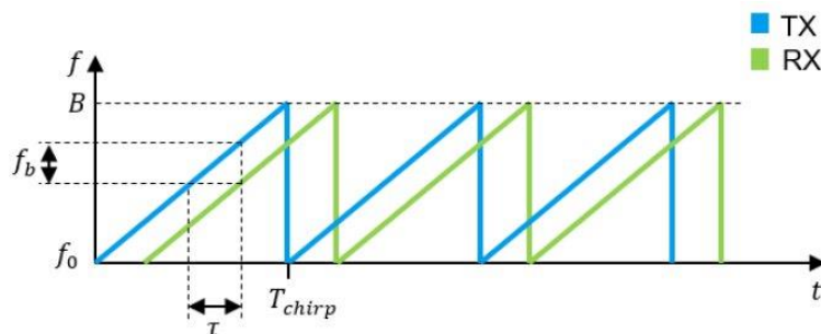
TX and RX FMCW radar signals using Sawtooth modulation signal
