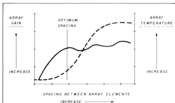
fig. 13. Array gain and array temperature versus spacing.
