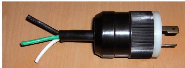
Figure 57 - Three wire plug. The green wire is ground. Photo by N5IUT
