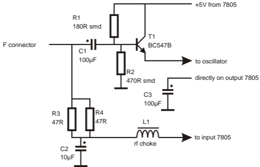
Schematics modulator
