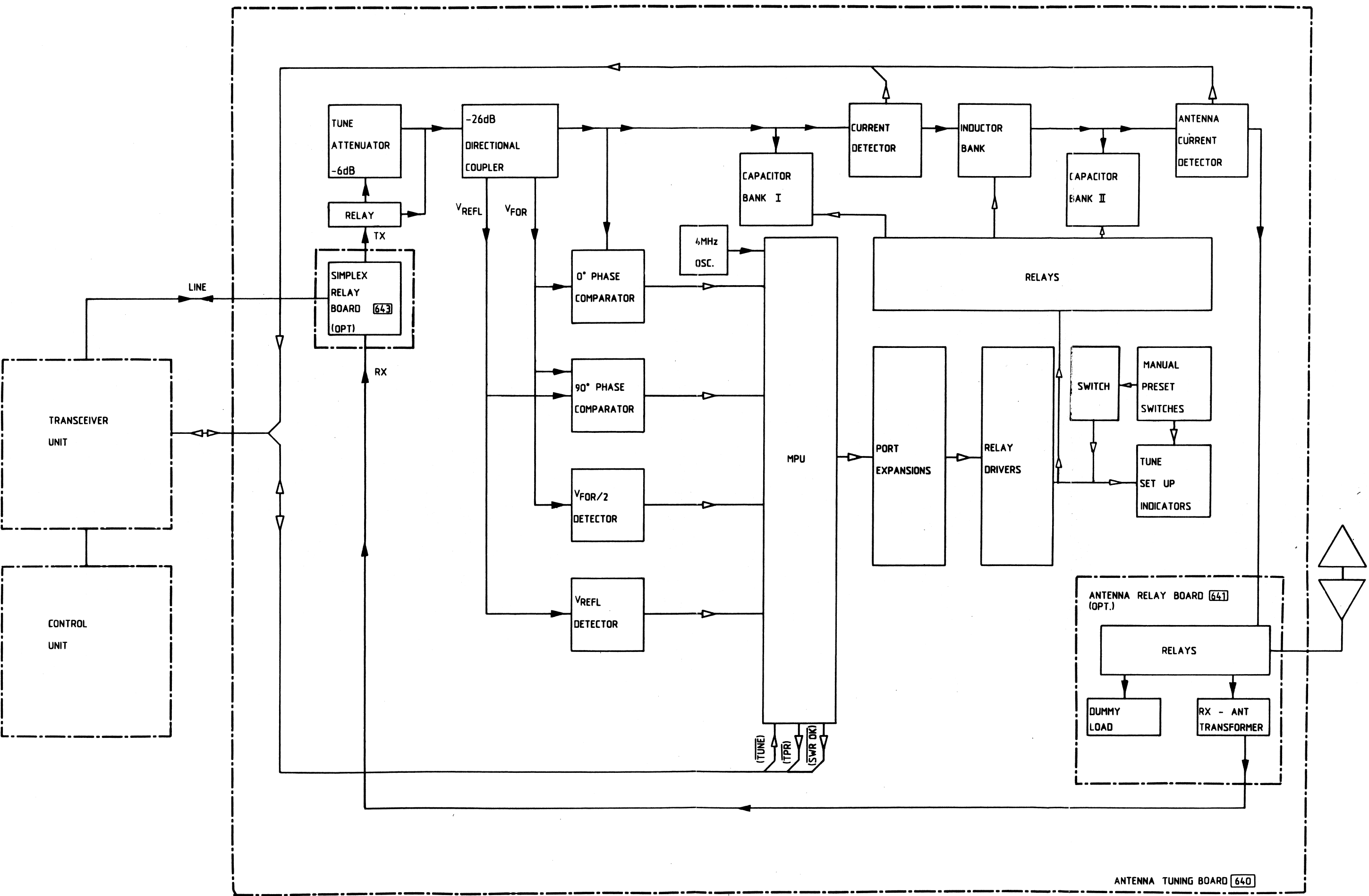
TRP 8250 S BLOCK DIAGRAM, ANTENNA TUNING UNIT VERSION 1A.
