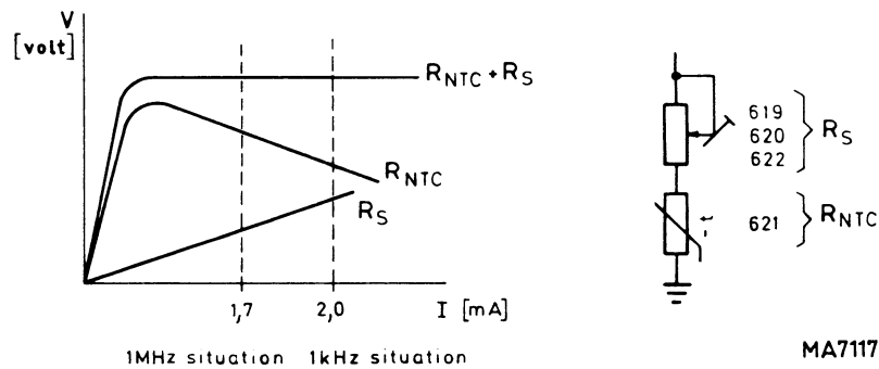
Fig. 8. Thermistor circuit
