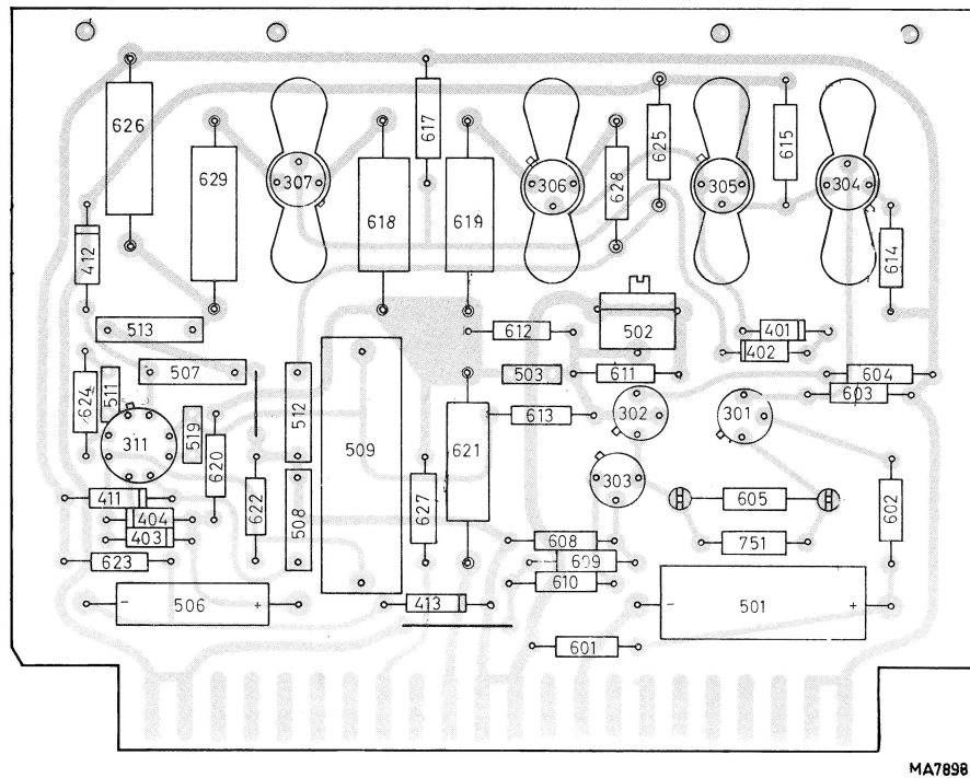
Fig. 18. Printed wiring board of amplifier
