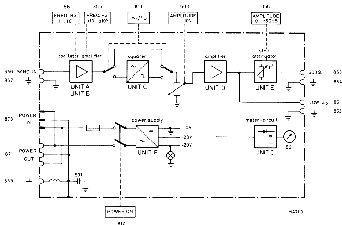
Fig. 4. Block diagram
