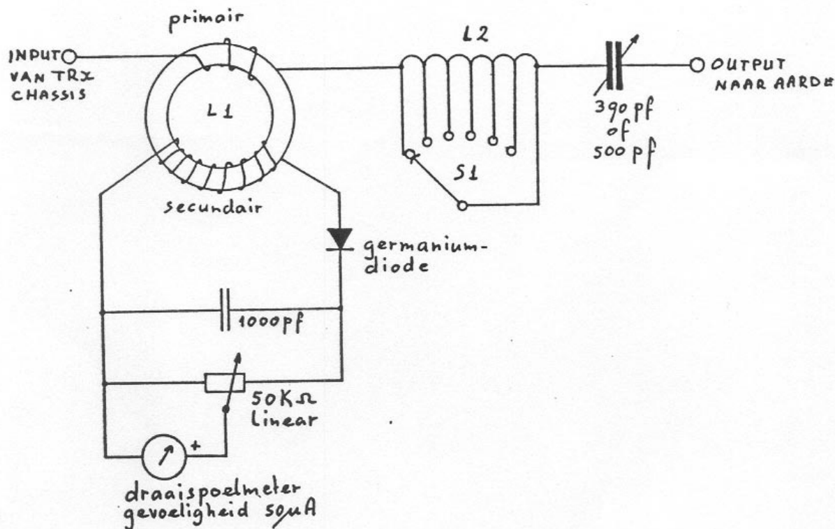
Schematics of the Artificial Ground
