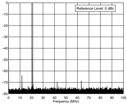
Kenwood TS-570D S/N: 80600403 21.0 MHz Band, Spectral Purity, 100 W P:\TESTS\TS570\TS570S15.TXT
