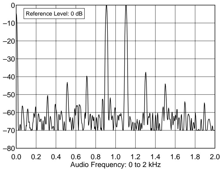
Kenwood TS-570D S/N: 80600403 14.020 MHz, AGC Slow, In-Band Receiver IMD P:\TESTS\TS570\TS570IBS.TXTWed Jan 22 18:15:59 1997
