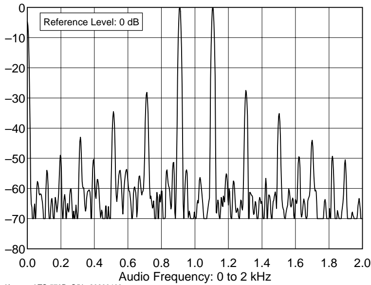
Kenwood TS-570D S/N: 80600403 14.020 MHz, AGC Fast, In-Band Receiver IMD P:\TESTS\TS570\TS570IBF.TXTWed Jan 22 18:16:55 1997
