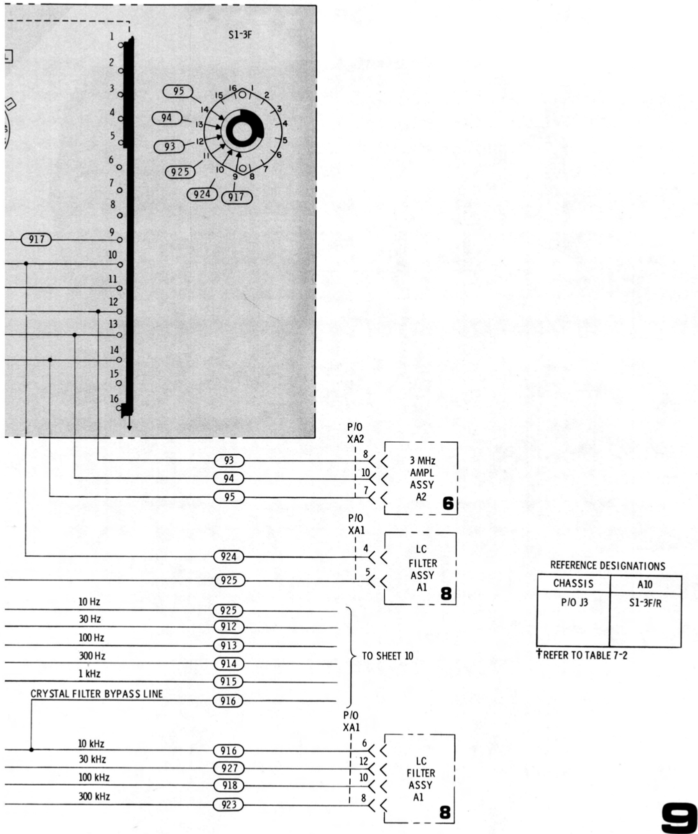
Figure 8-30. Amplifier/Filter Control Circuits
