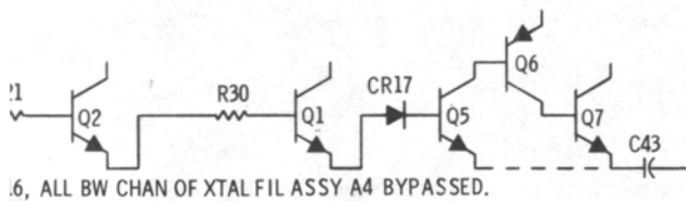
SIGNAL FLOW PATH
