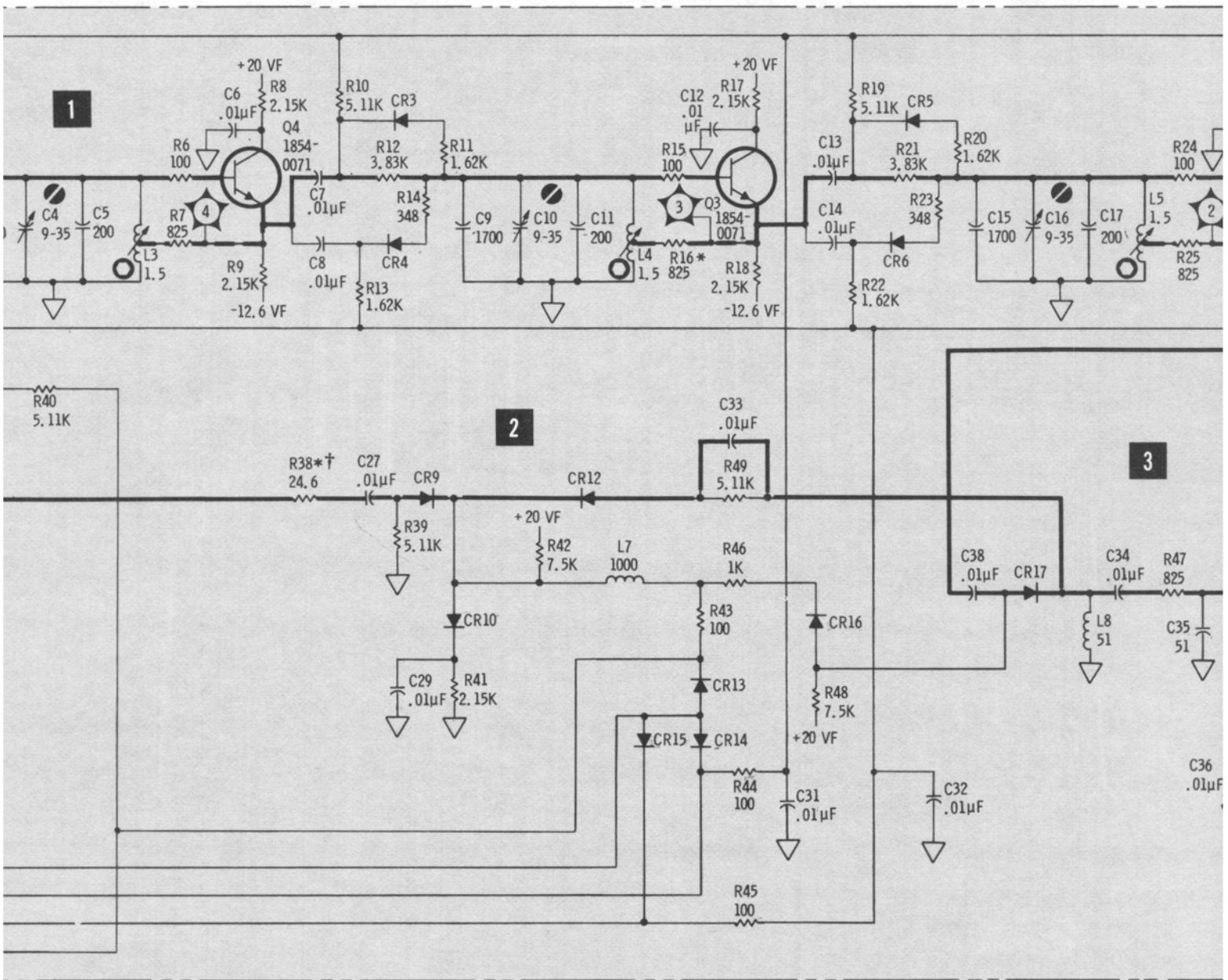
SIGNAL FLOW PATH
