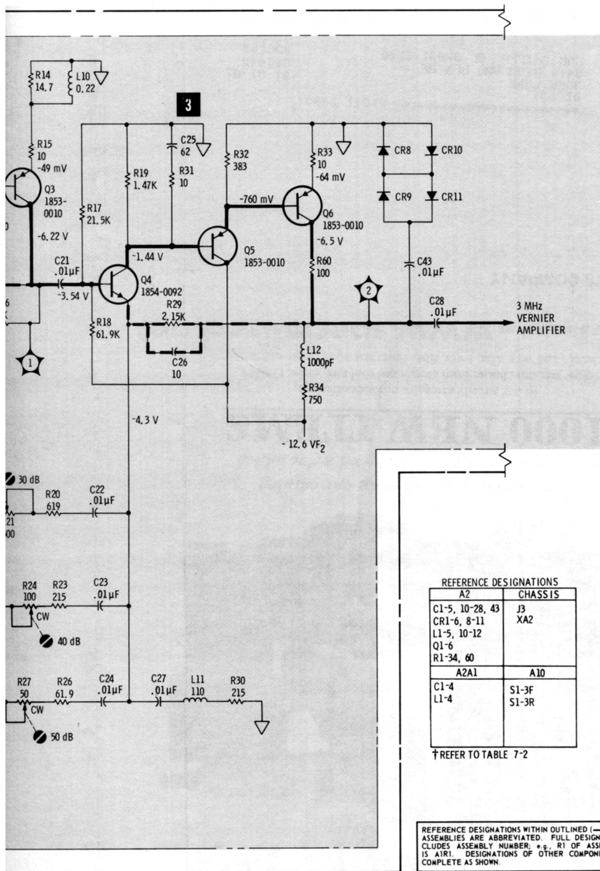
Figure 8-25. 3 MHz Amplifier (1 of 2)
