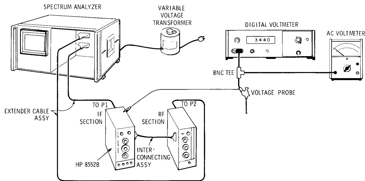
Figure 5-1. Power Supply Check and Adjustment Test Setup
