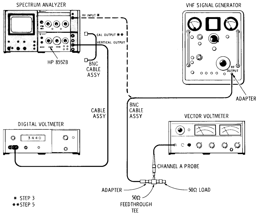
Figure 4-3. Calibrator Amplitude Test Setup
