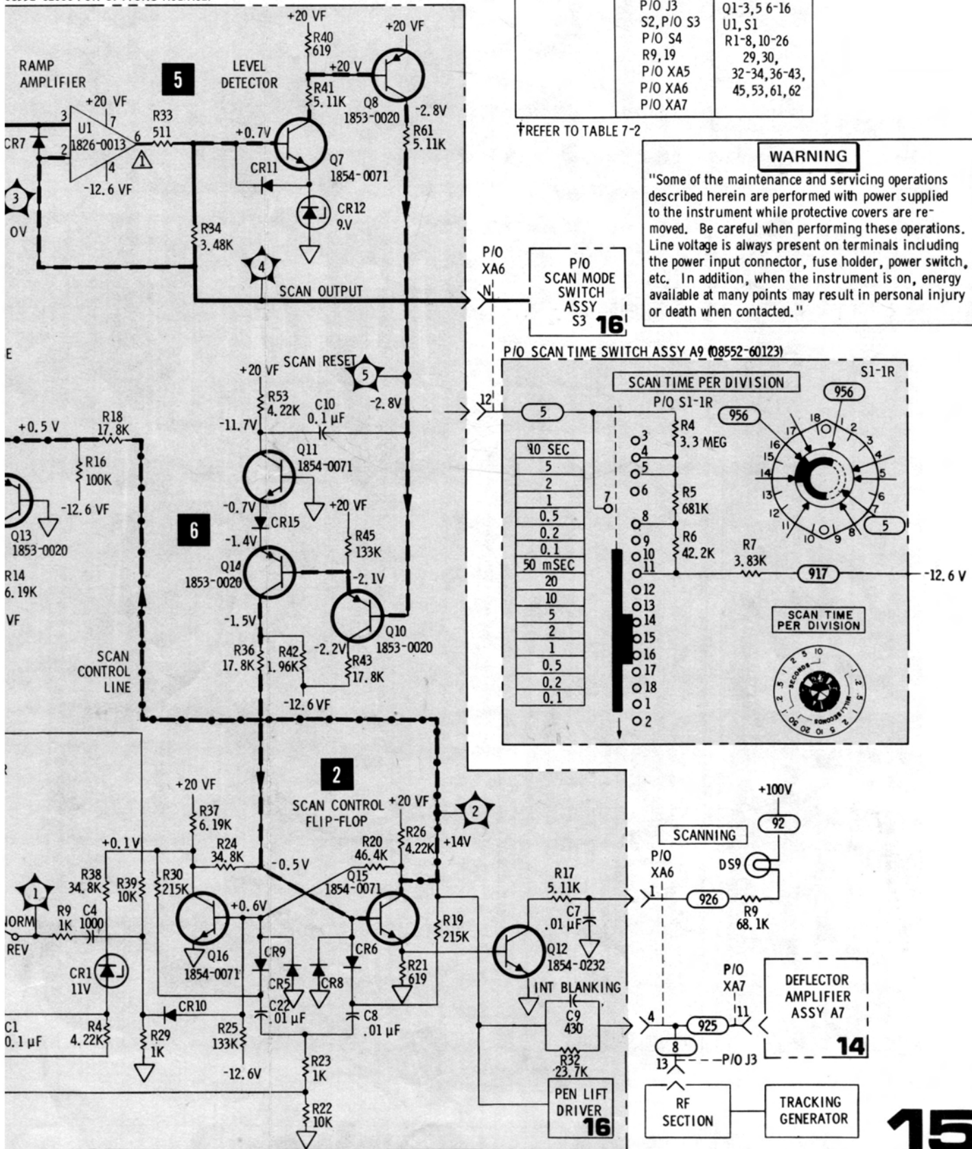
Figure 8-43. Scan Generator and Trigger Circuits
