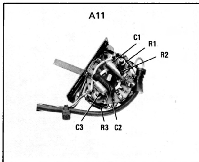
Figure 8-11. Video Filter Assembly A11
