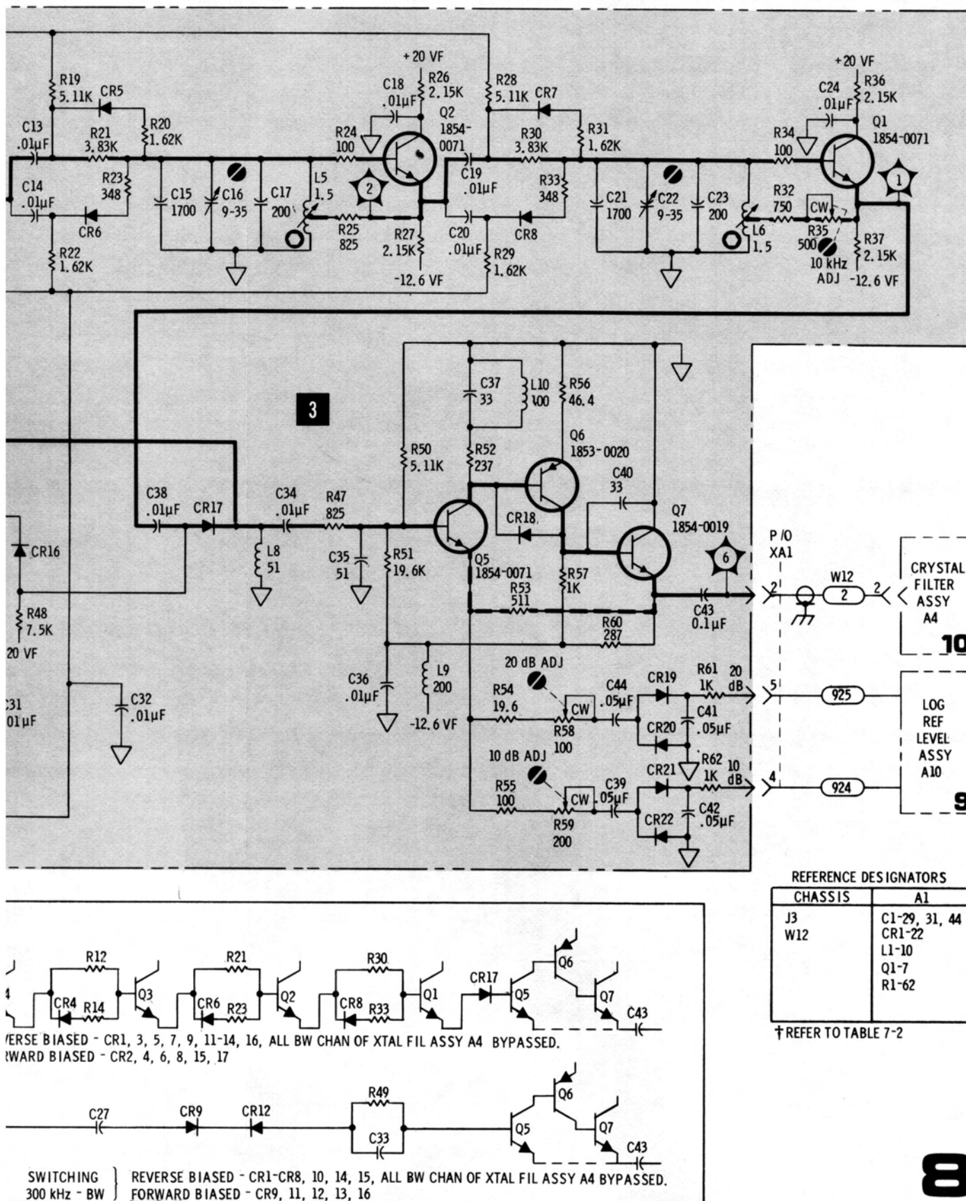
Figure 8-29. LC Bandwidth Filter
