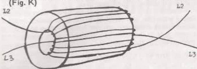
Transformer L2:L3 wound on FX1115 ferrite bead. (Fig. K)
