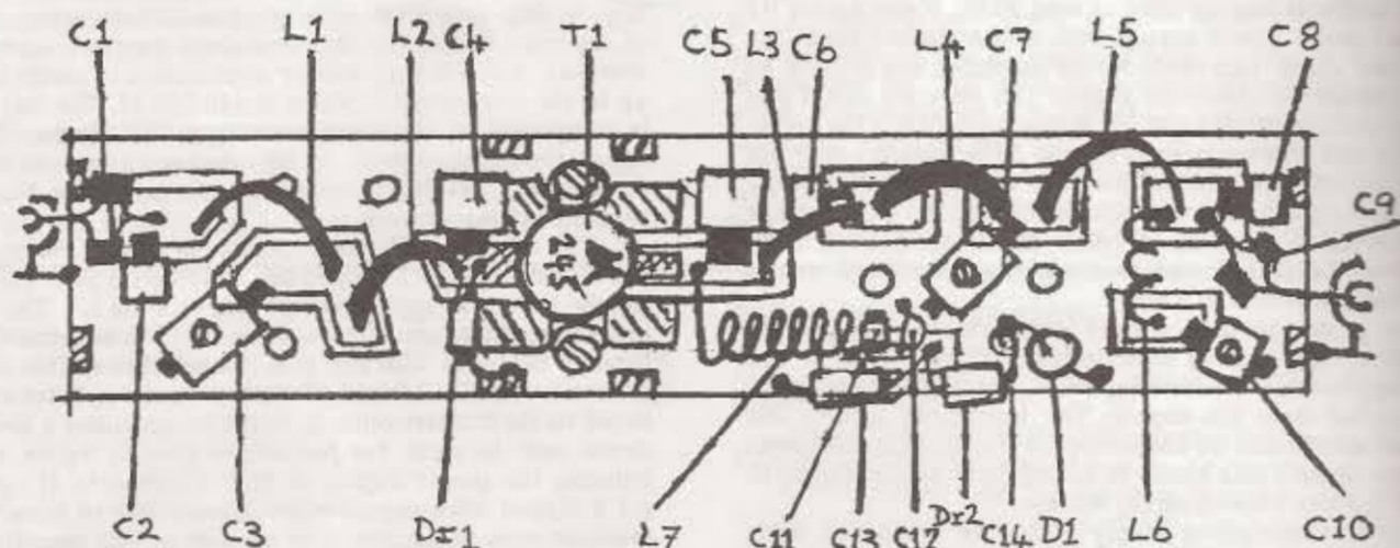
LAYOUT WITH ISLANDS FIG. N
