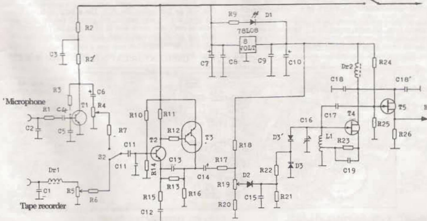
TRANSMITTER CIRCUIT DIAGRAM
