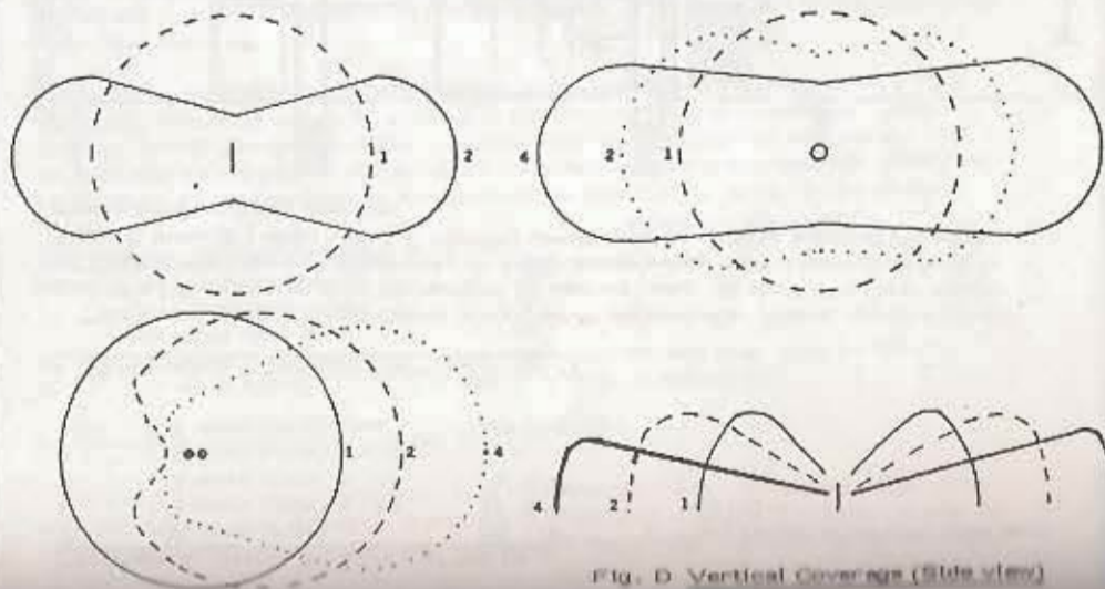
Fig. D Vertical Coverage (Side view)
