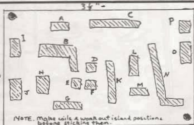
Actual Size 2-1/8" x 3-1/8" with islands for ½WATT DRIVER STAGE (Fig 2).
