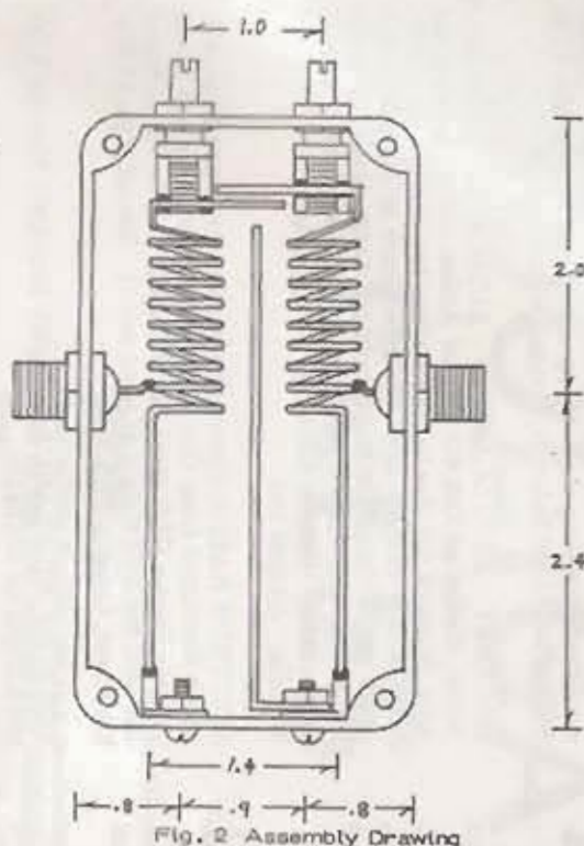
Fig. 2 Assembly Drawing
