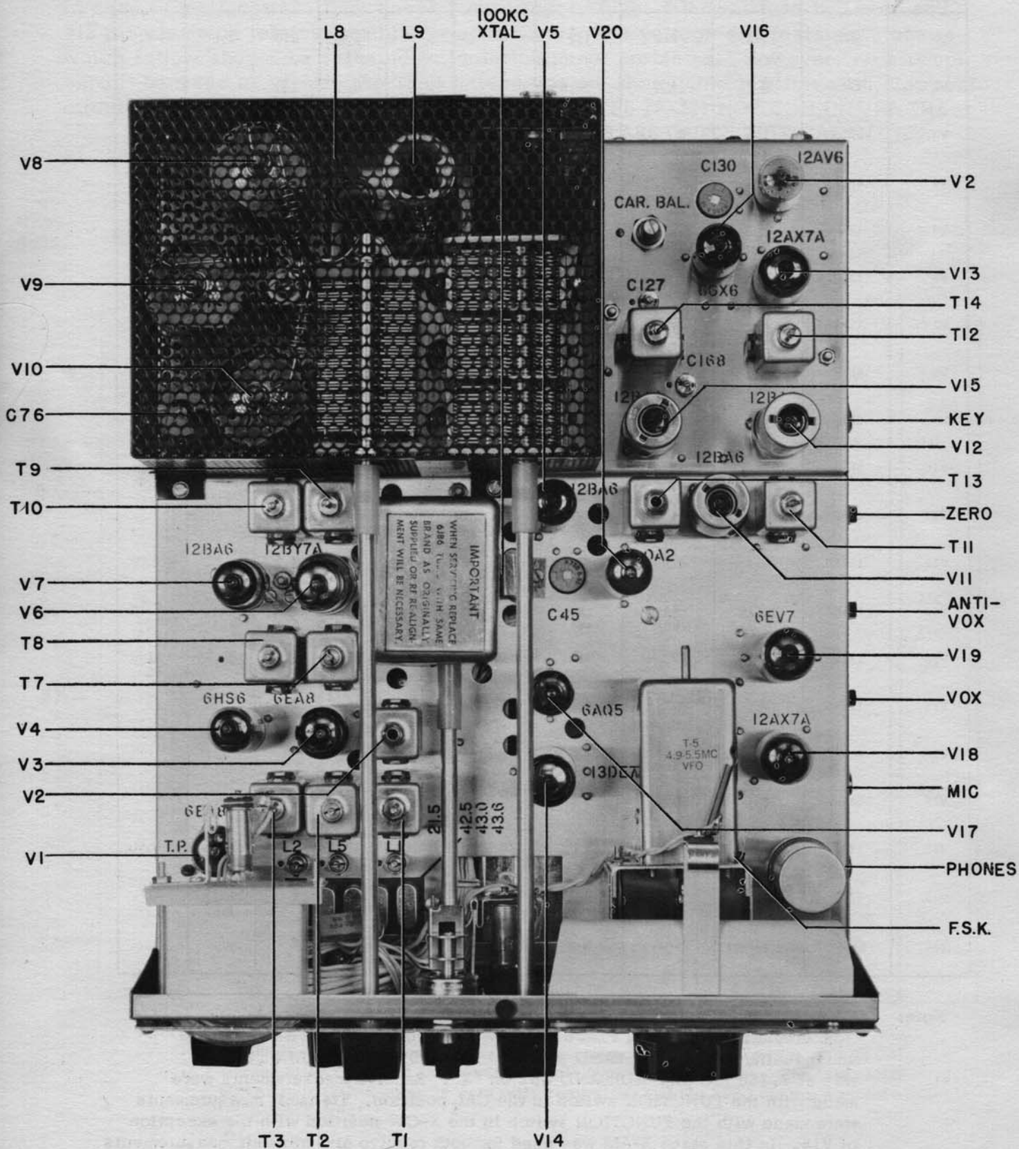
Fig. 13 TOP VIEW
