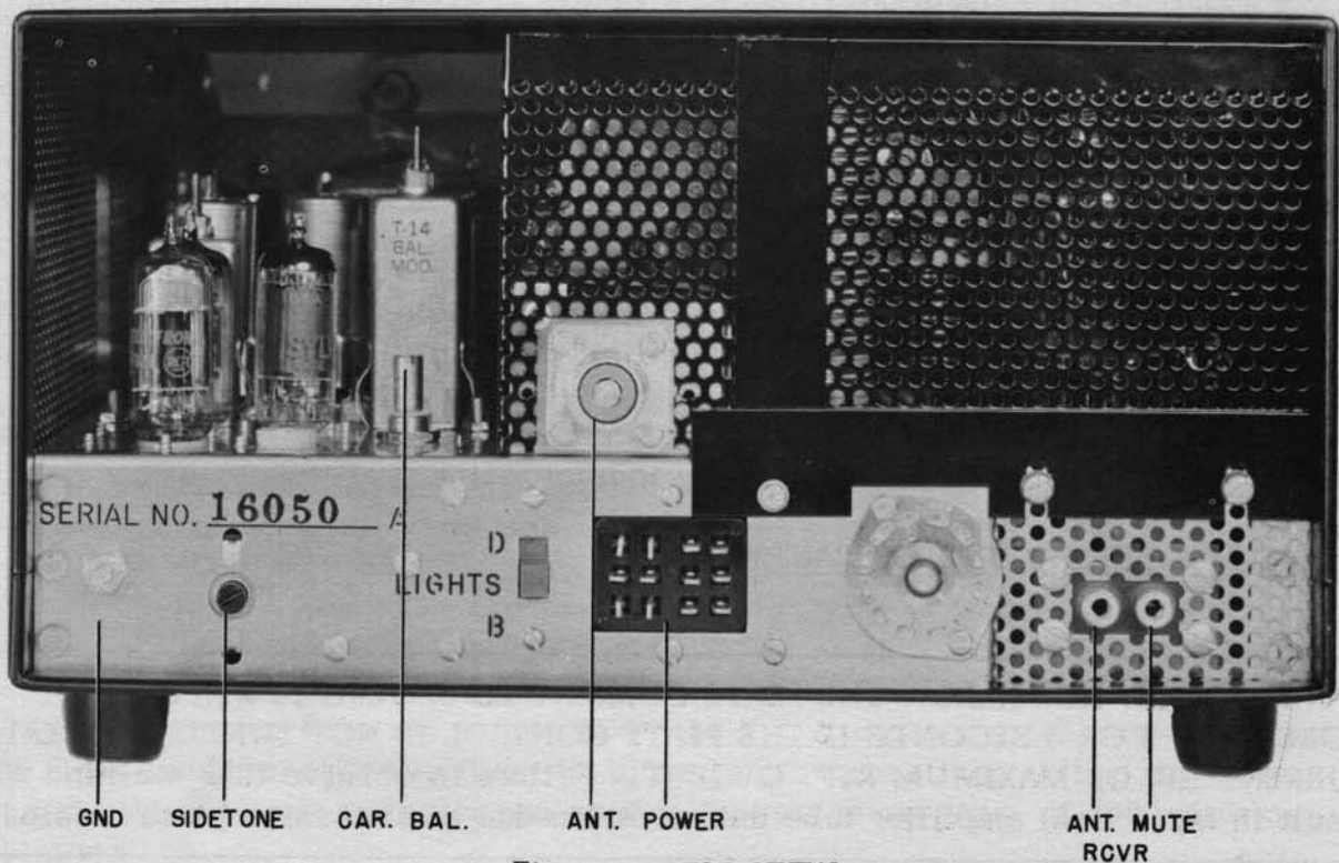
Fig. 7 REAR VIEW
