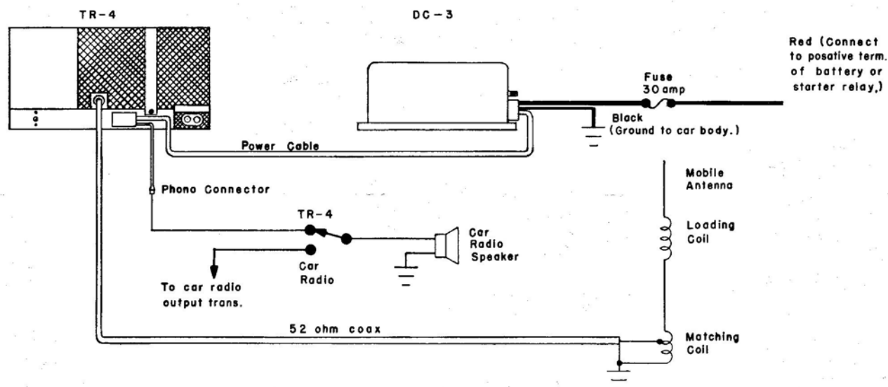
FIG. 4 ELECTRICAL CONNECTIONS FOR MOBILE INSTALLATION OF TR-4
