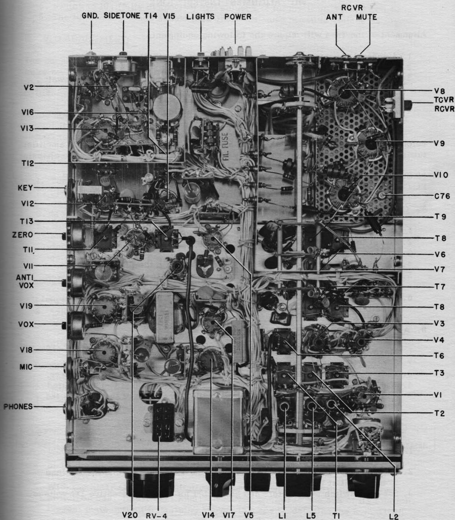
Fig. 14 BOTTOM VIEW
